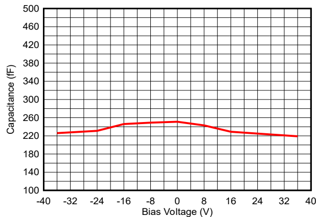
図 5-1. Bias Voltage vs Capacitance
