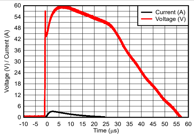
図 5-4. 8/20 μs Surge Response
