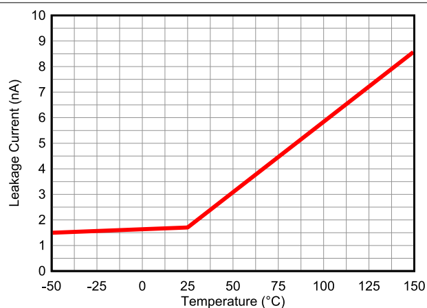
図 5-8. Leakage Current vs Temperature
