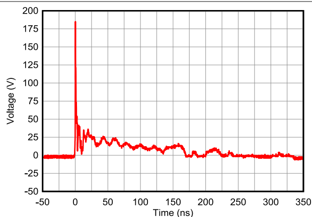
図 5-3. +8kV Clamped IEC Waveform
