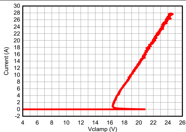
図 5-5. Positive TLP Curve
