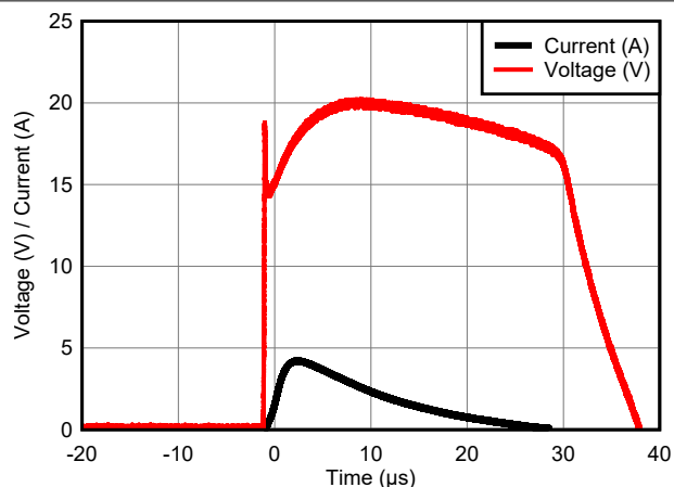
図 5-2. 8/20μs Surge Response
