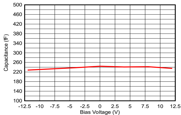
図 5-1. Bias Voltage vs. Capacitance
