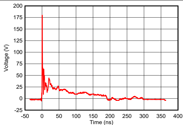
図 5-5. +8kV Clamped IEC Waveform
