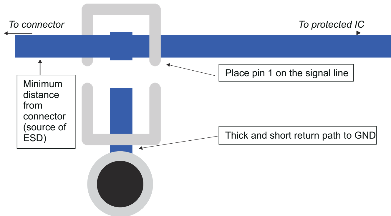
✎ 10-1. Layout Recommendation
