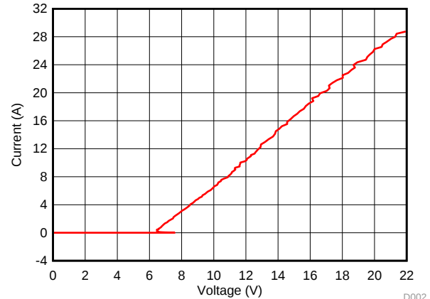
图 2. Negative TLP Curve, Connector side IO Pin to GND (Plotted as positive TLP from GND to IO, t_p=100\text{ns} )
