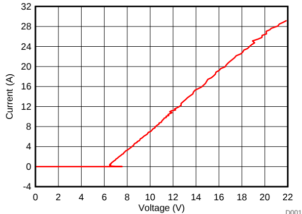
图 1. Positive TLP Curve, Connector side IO Pin to GND ( t_p=100\text{ns} )
