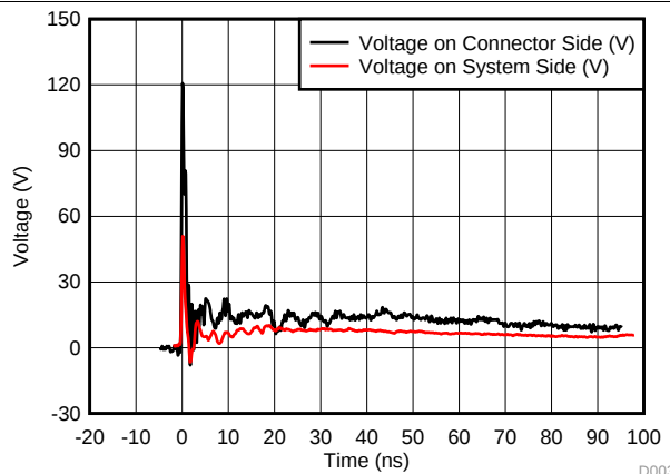
图 3. Clamping voltage waveform for +8kV IEC 61000-4-2 stress. See 图 11 for details.
