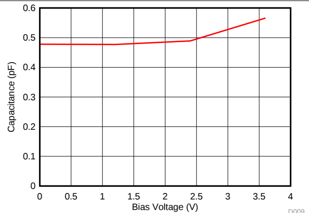
图 6. Capacitance vs. Bias Voltage at 25 degree Celsius
