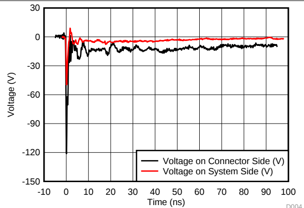
图 4. Clamping voltage waveform for -8kV IEC 61000-4-2 stress. See 图 11 for details.
