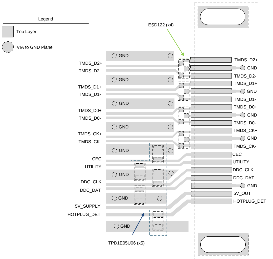
Figure 20. HDMI2_Layout
