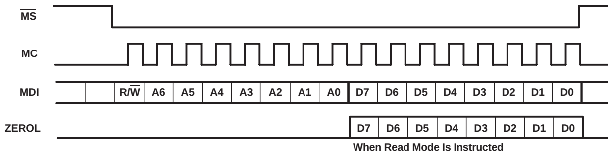
Figure 29. Control Data Word Format for MDI
