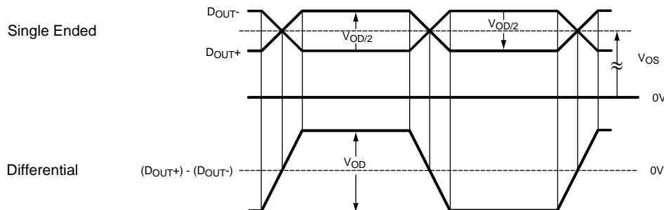
FIG 1. Serializer V_{OD} Output
