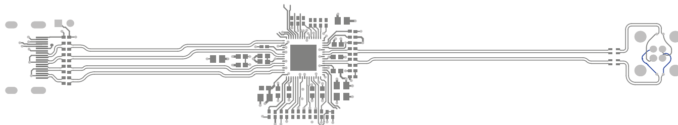
Figure 32. DS90UH949A-Q1 Serializer Layout Example
