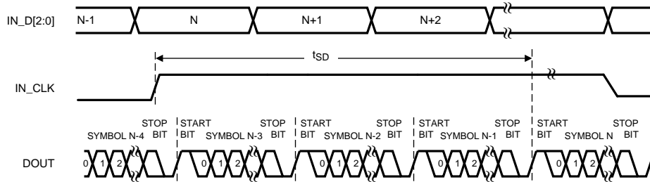
图 4. Latency Delay
