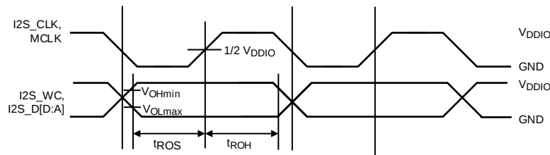
☒ 6. Output Data Valid (Setup and Hold) Times
