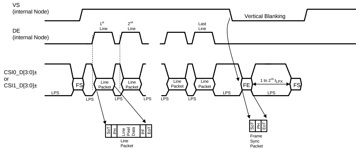
FIG 13. Long Line Packets and Short Frame Sync Packets
