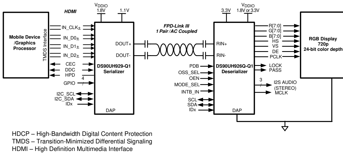
Figure 23. Typical System Diagram
