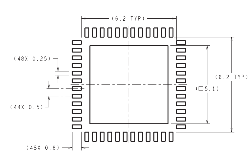
Figure 45. 48-Pin WQFN Stencil Example of Via and Opening Placement
