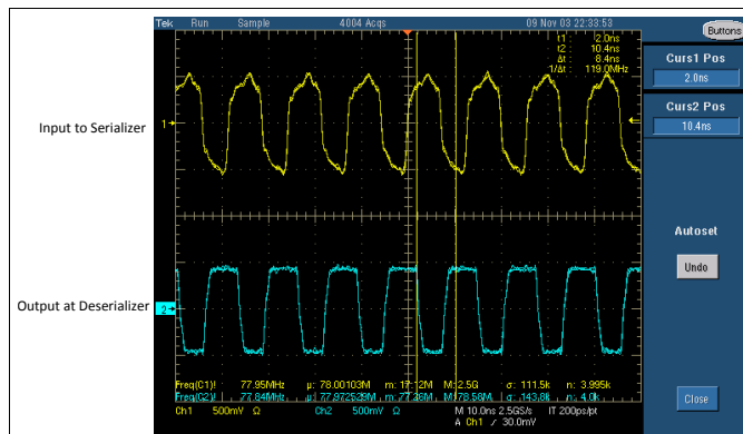
Figure 41. 78-MHz Clock at Serializer and Deserializer
