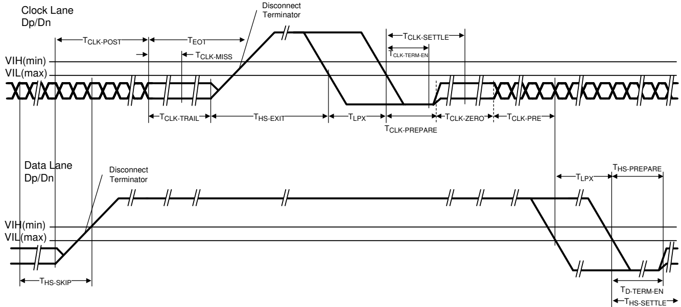
図 4-6. Switching the Clock Lane Between Clock Transmission and Low-Power Mode
