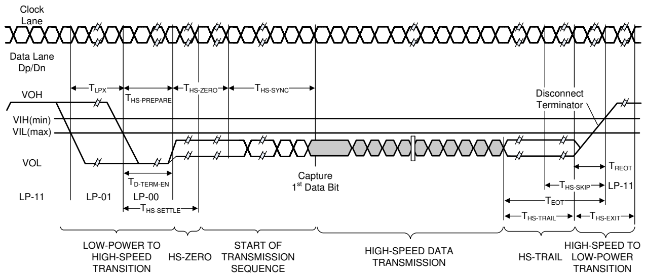
図 4-7. High-Speed Data Transmission Burst
