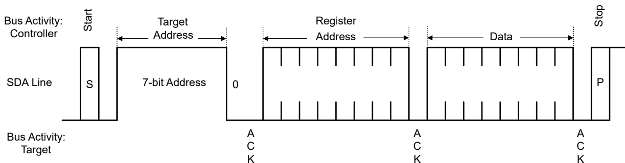
図 7-21. Serial Control Bus — WRITE
