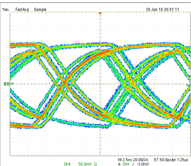
図 6-12. Typical 50 Mbps Back Channel Output Waveform
