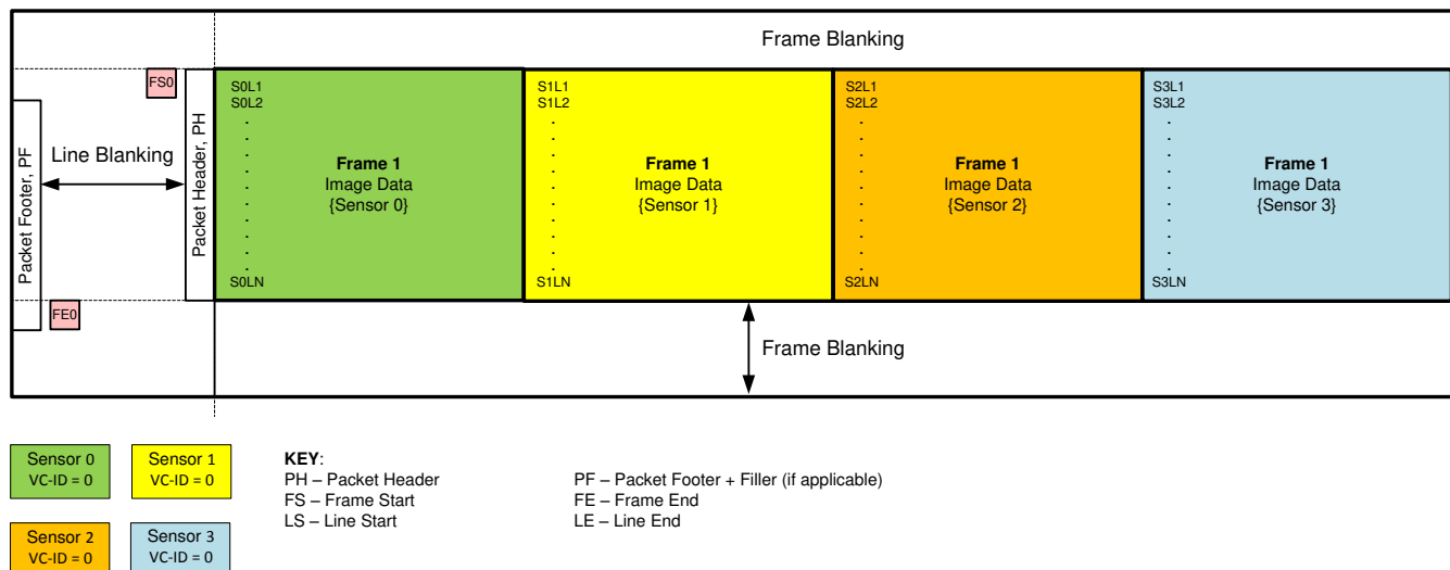
图 7-17. Line-Concatenated Format
