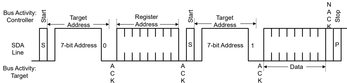
図 7-20. Serial Control Bus — READ
