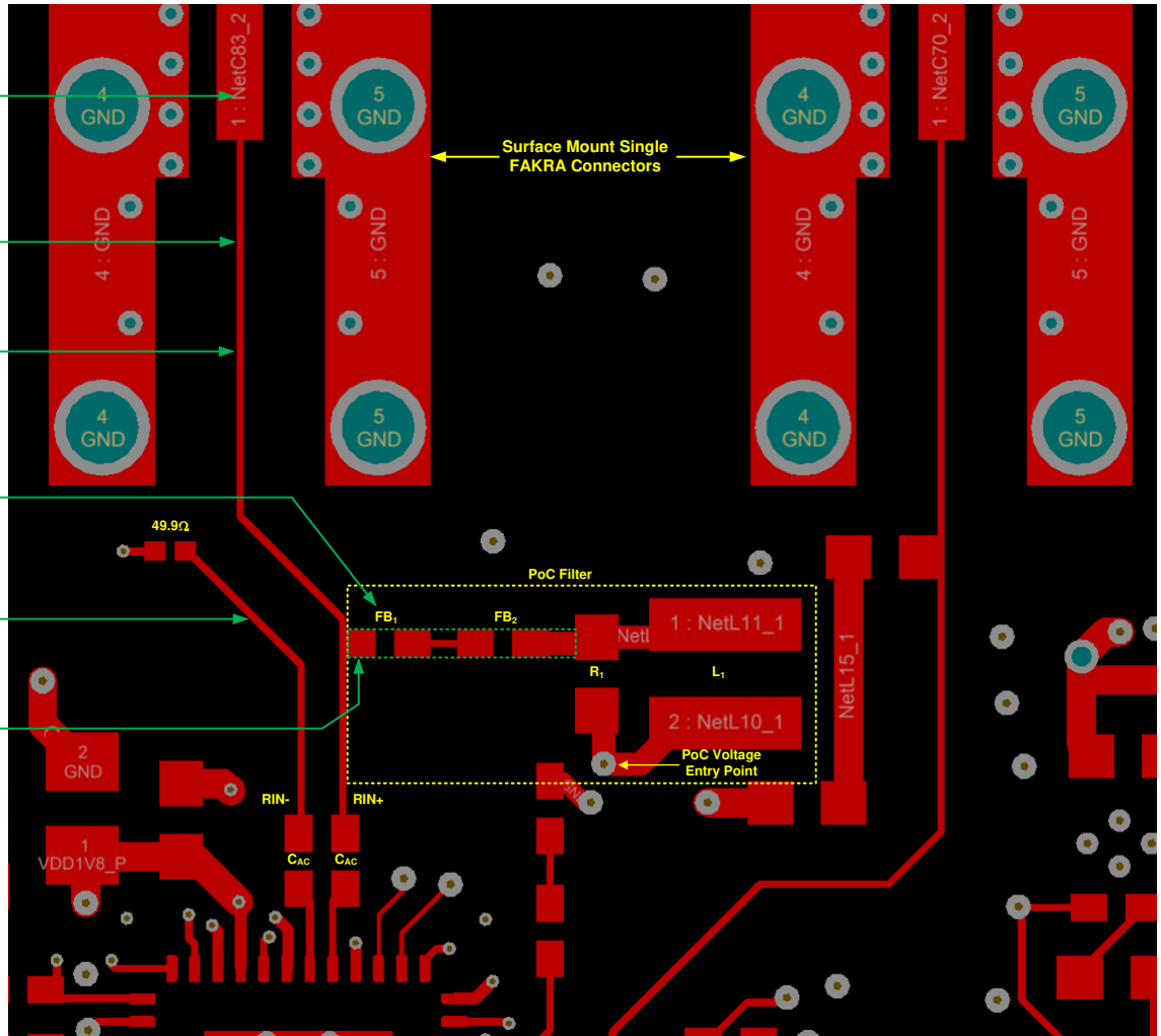
❏ 8-18. Example Routing of FPD-Link III Traces to a Single Mini-Fakra Connector and PoC Components
