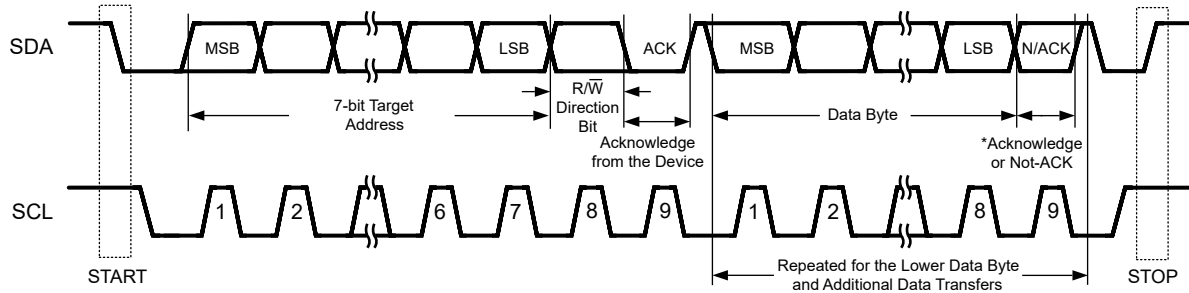
図 7-22. Basic Operation
