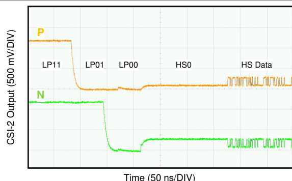
図 8-10. CSI-2 Start of Transmission (SoT)
