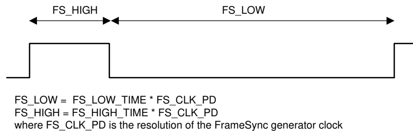
図 7-14. Internal FrameSync Signal
