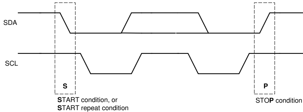
図 7-19. START and STOP Conditions
