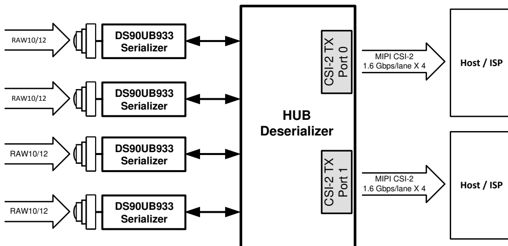
図 8-15. Four DS90UB933-Q1 Sensor Data Onto CSI-2 Over 2 Ports
