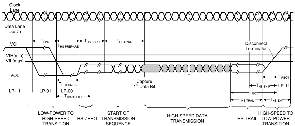
6-7. High Speed Data Transmission Burst
