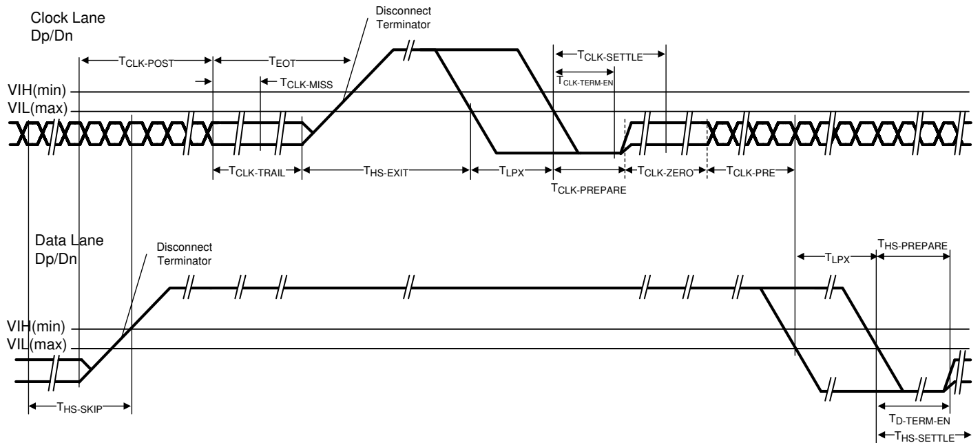
❏ 6-6. Switching the Clock Lane between Clock Transmission and Low-Power Mode
