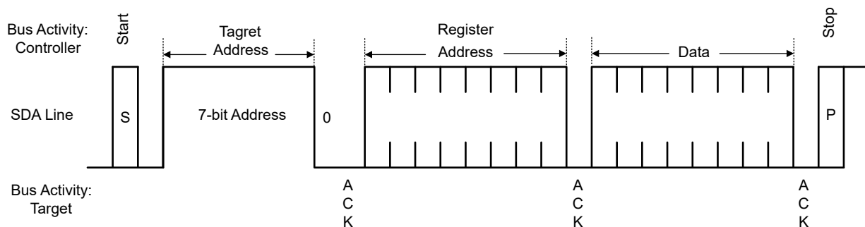
7-27. Serial Control Bus — WRITE
