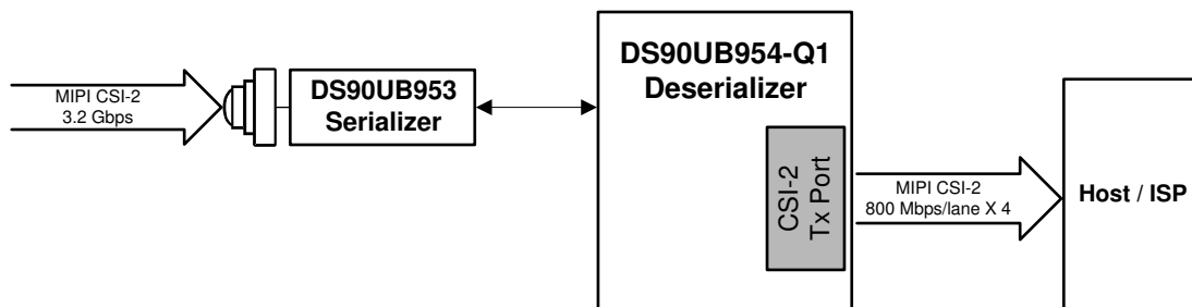
✎ 8-13. DS90UB953-Q1 Sensor Data to 1 Rx Port
