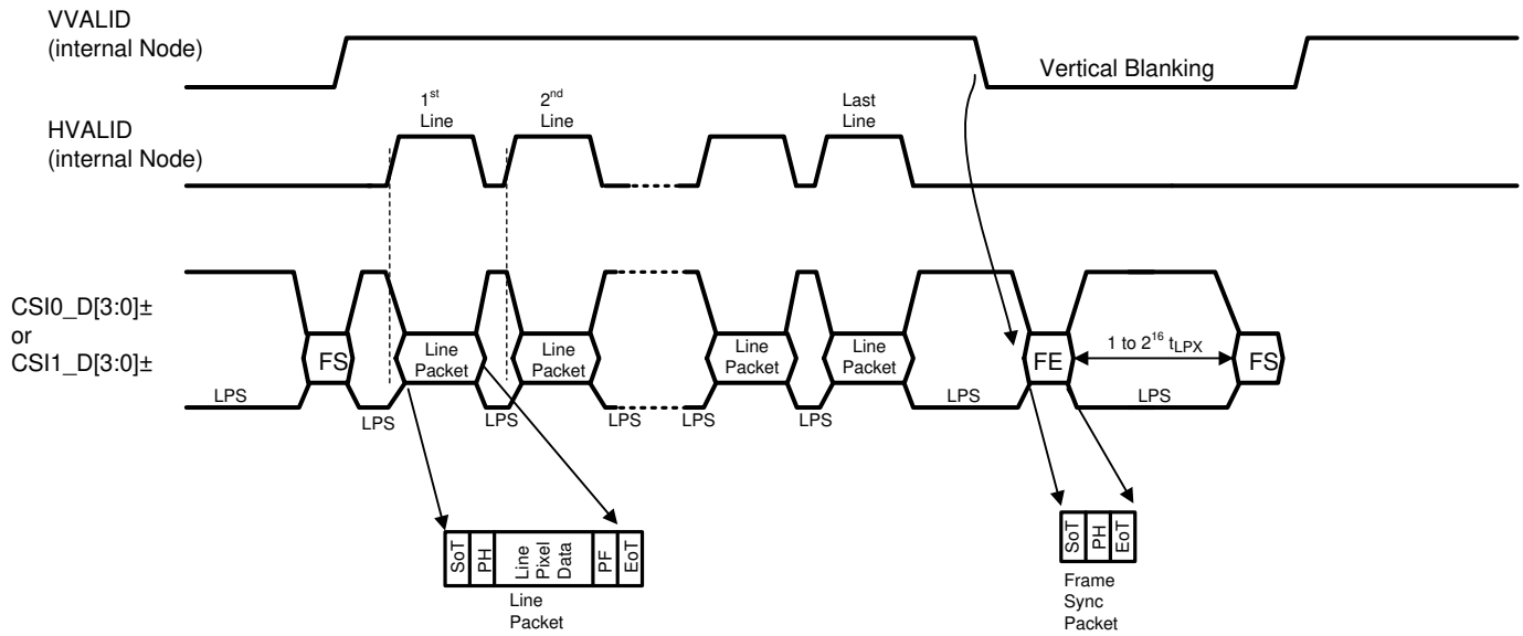
FIG 6-8. Long Line Packets and Short Frame Sync Packets
