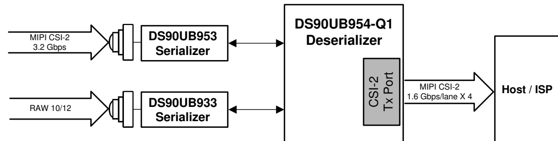
✎ 8-15. One DS90UB953-Q1 and One DS90UB933-Q1 Sensor Data Combined to One CSI-2 output
