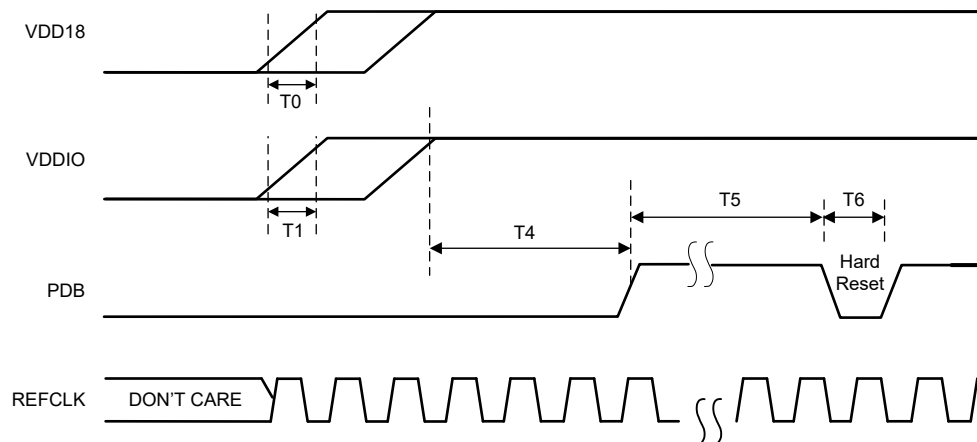
FIG 9-1. Power Supply Sequencing VDD_SEL = LOW, Internal VDD 1.1-V Supply
