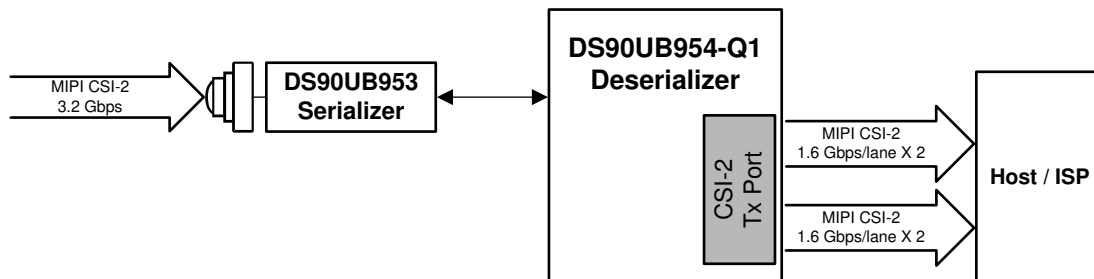
✎ 8-14. DS90UB953-Q1 Sensor Data Replicated onto 2x 2-Lane CSI-2
