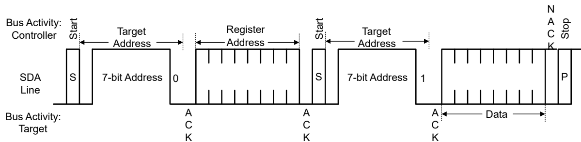
7-26. Serial Control Bus — READ
