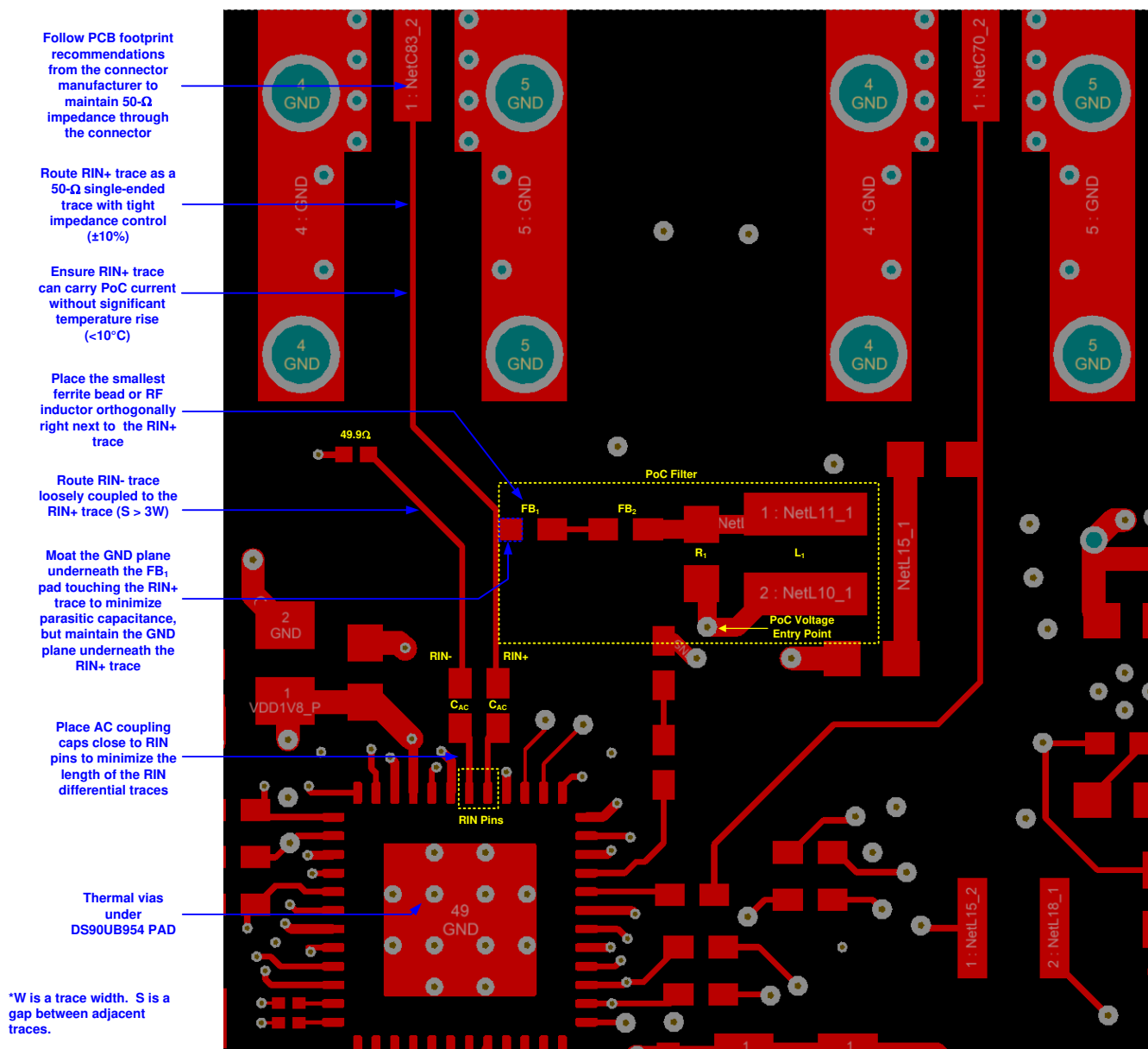
FIG 10-1. DS90UB954-Q1 PCB Layout Example: FPD-Link III Signal Traces and PoC Filter
