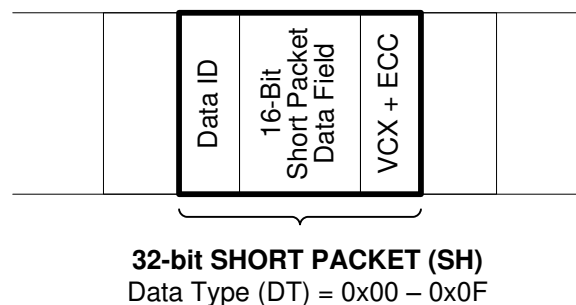
☒ 7-9. CSI-2 Short Packet Structure
