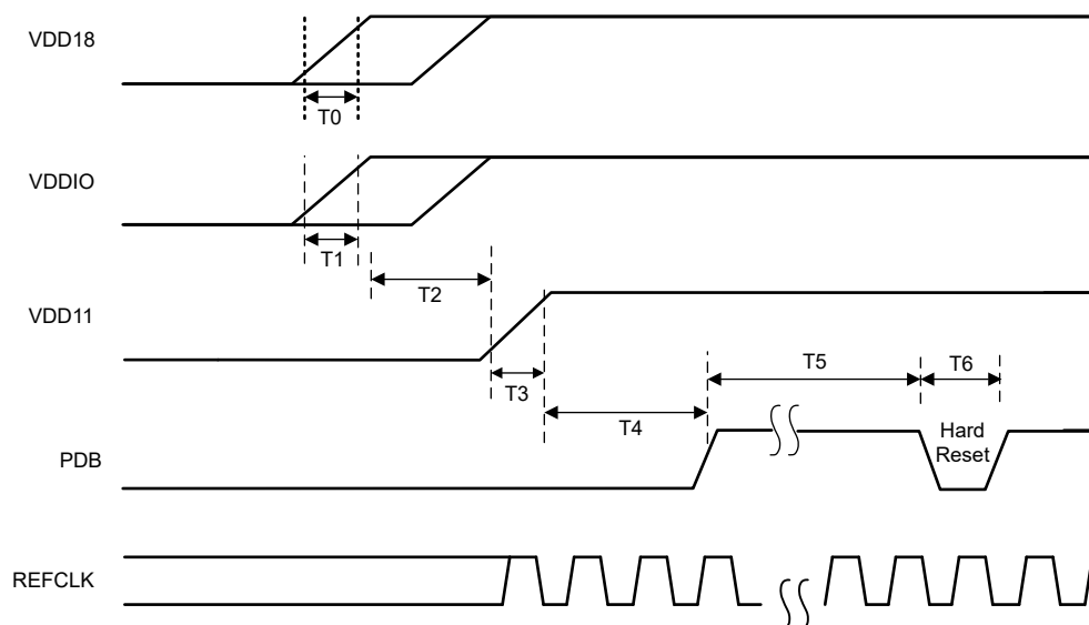
FIG 9-2. Power Supply Sequencing VDD_SEL = HIGH, External VDD 1.1-V Supply
