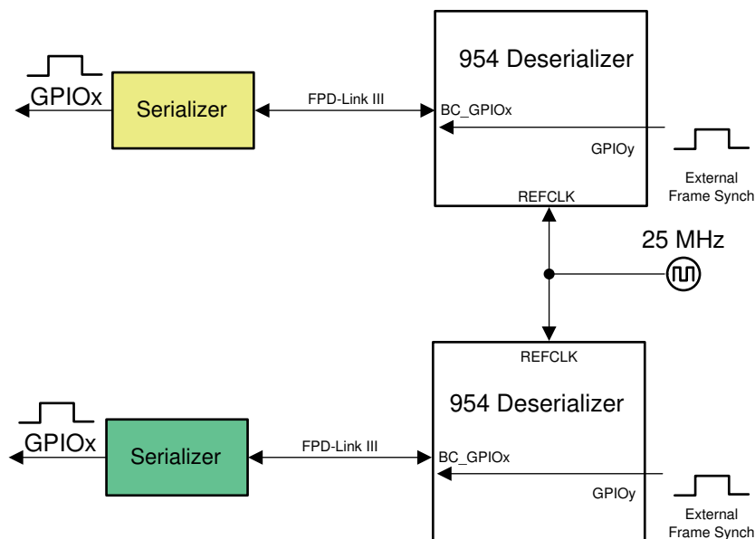
7-18. External FrameSync With Two DS90UB954 Deserializers
