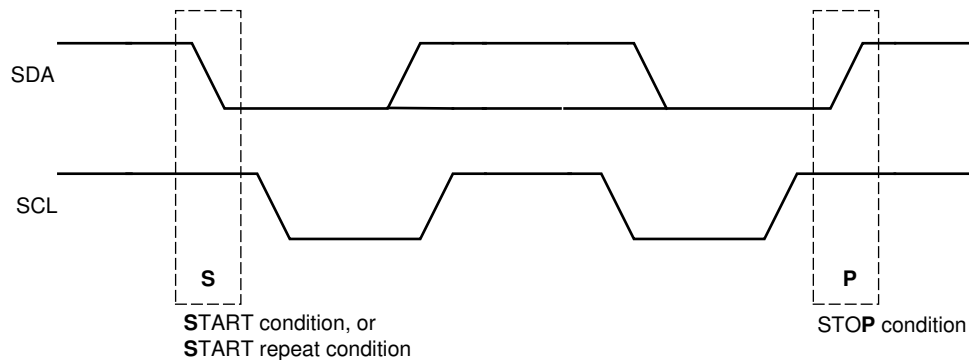
7-25. START and STOP Conditions
