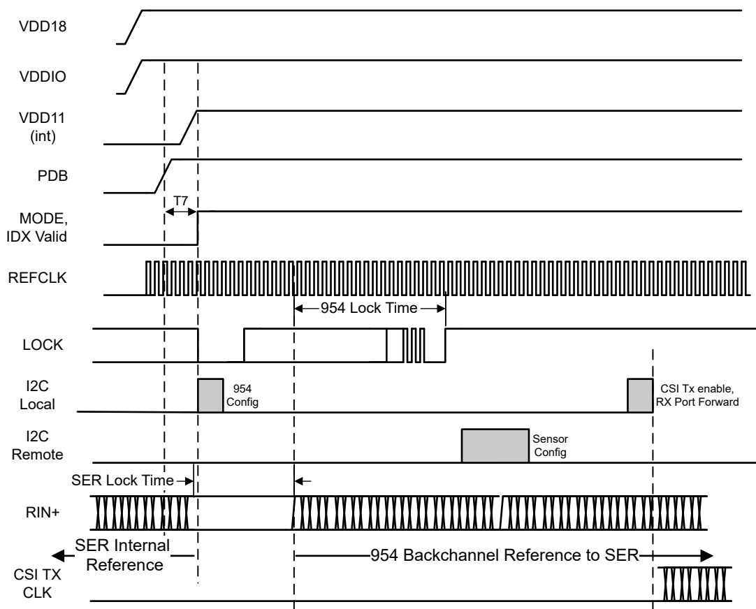
FIG 9-3. Power-Up Sequencing Synchronous Back Channel Clocking Mode, VDD_SEL = LOW
