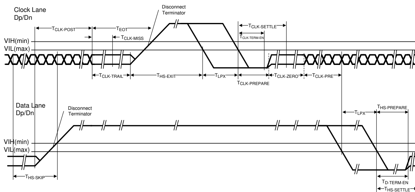
6-7. Switching the Clock Lane Between Clock Transmission and Low-Power Mode
