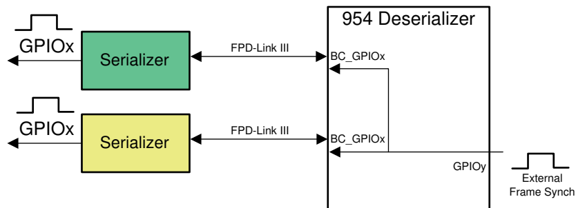
7-17. External FrameSync
