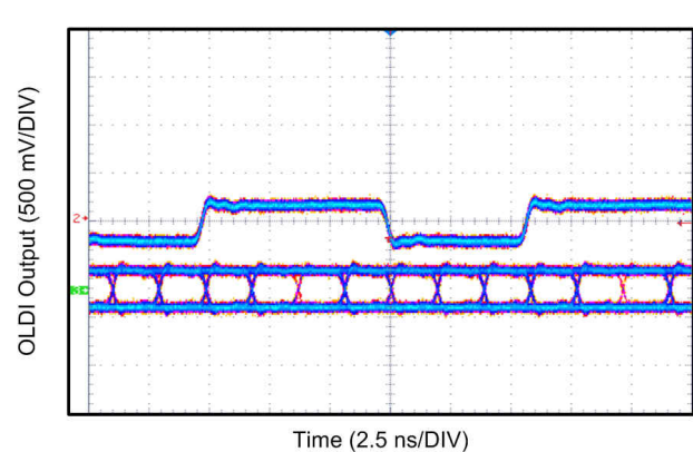
8-7. OpenLDI Clock and Data Output at 74.25-MHz Pixel Clock
