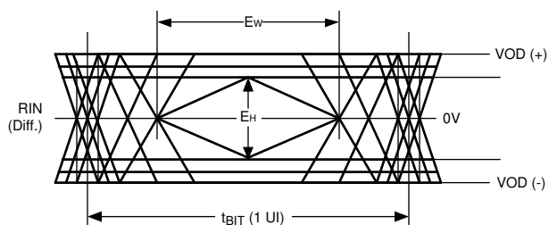
FIG 6-2. CML Output Driver
