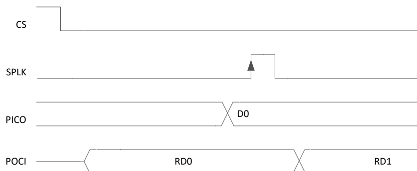
FIG 7-3. Forward Channel SPI Read
