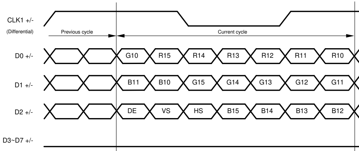
FIG 7-25. 18-Bit Color Single FPD-Link Mapping, Standard 18 Bit (MAPSEL = L)
