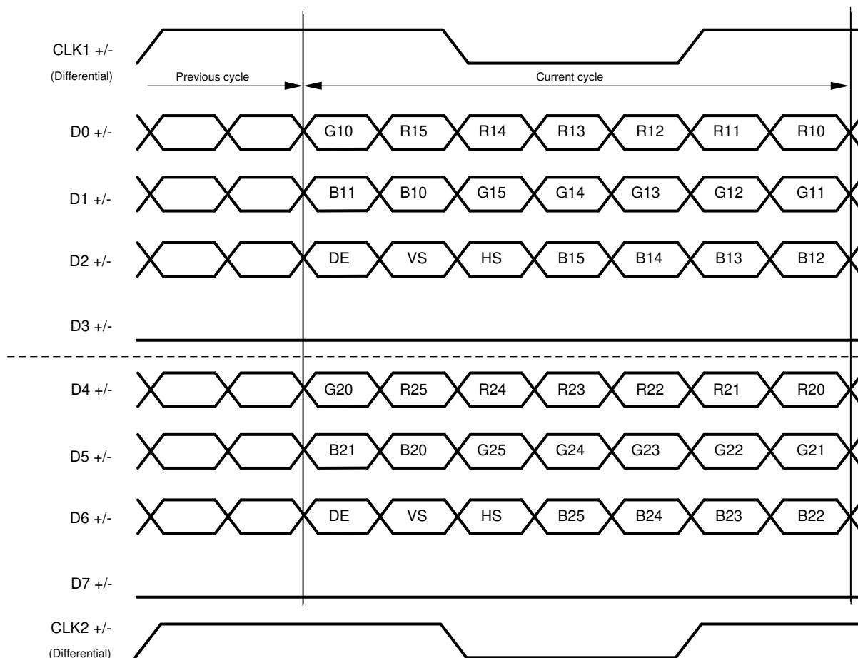
FIG 7-23. 18-Bit Color Dual FPD-Link Mapping, Standard 18 Bit (MAPSEL = L)
