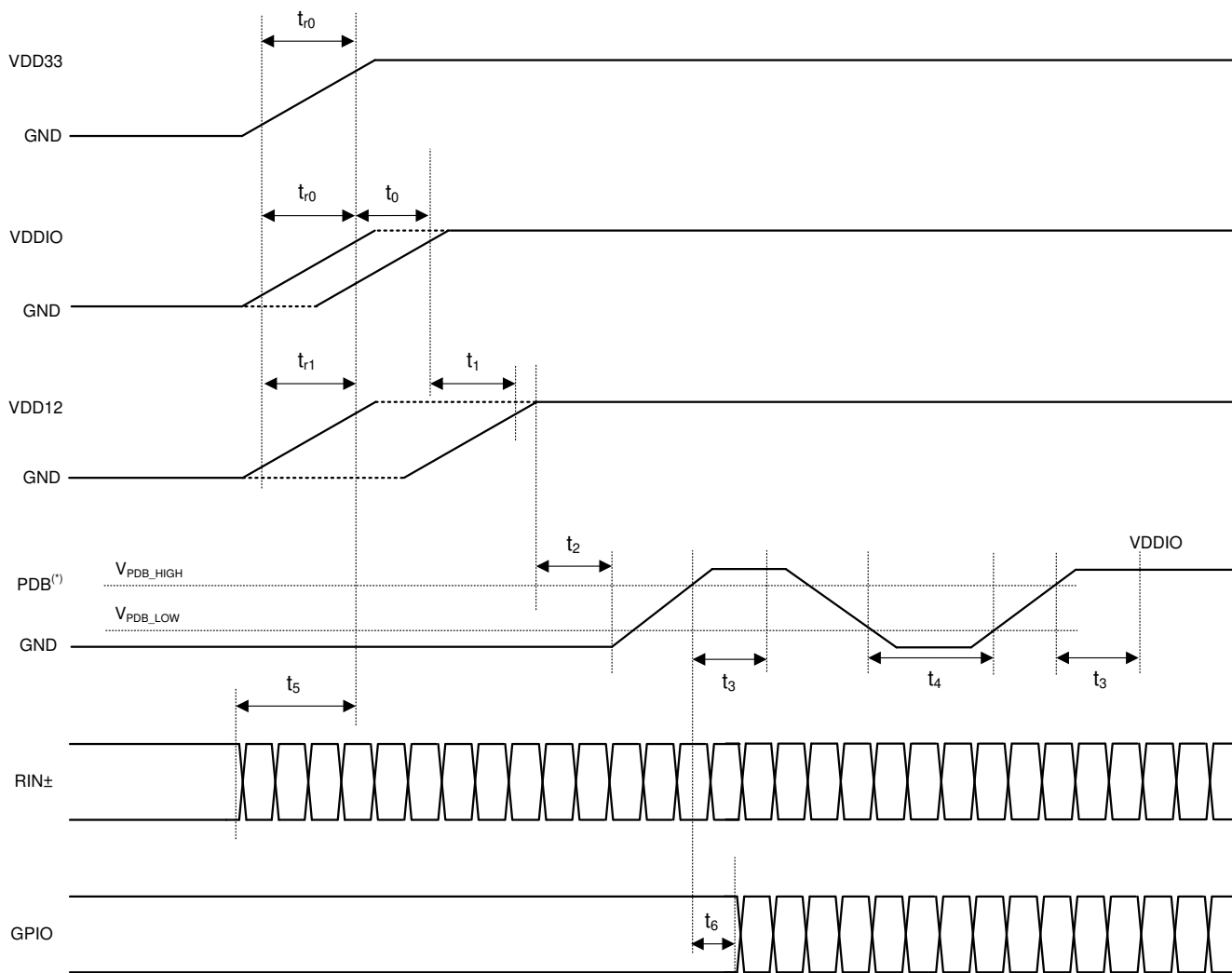
图 9-1. Power Sequence
