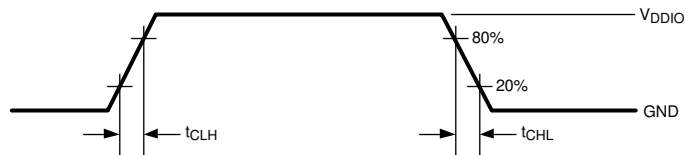
FIG 6-3. LVCMOS Transition Times
