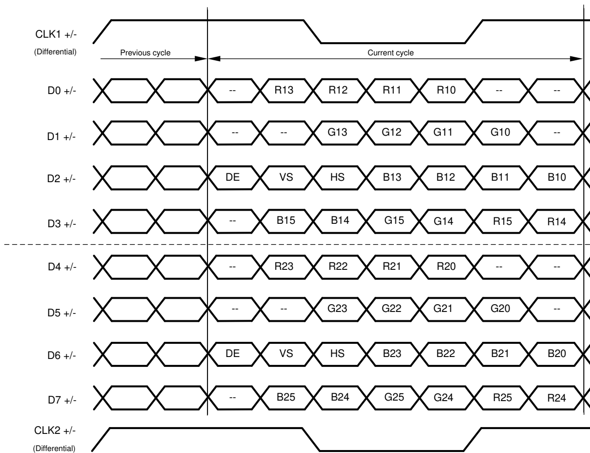
FIG 7-22. 18-Bit Color Dual FPD-Link Mapping, "4 Lane 18 Bit Mode" (MAPSEL = H)
