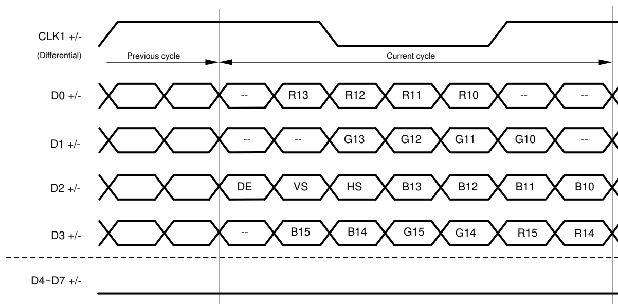
FIG 7-24. 18-Bit Color Single FPD-Link Mapping, "4 Lane 18 Bit Mode" (MAPSEL = H)
