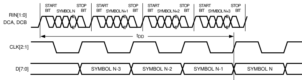
FIG 6-4. Latency Delay
