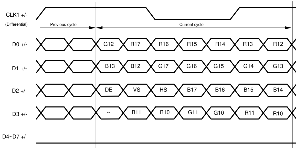
FIG 7-21. 24-Bit Color Single FPD-Link Mapping: LSBs on D3, "JEIDA" (MAPSEL = L)
