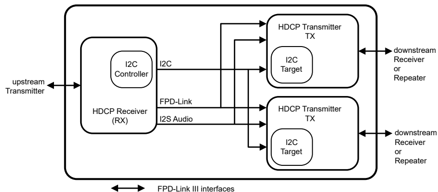
FIG 7-10. 1:2 Repeater Configuration
