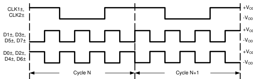
FIG 6-1. Checkerboard Data Pattern
