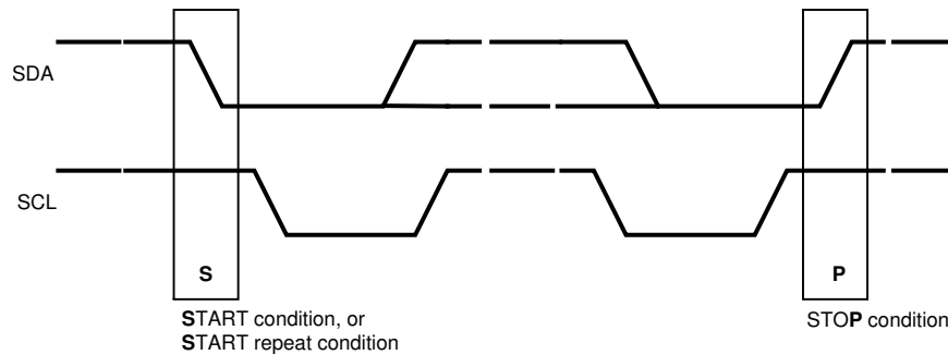
FIG 7-29. START and STOP Conditions
