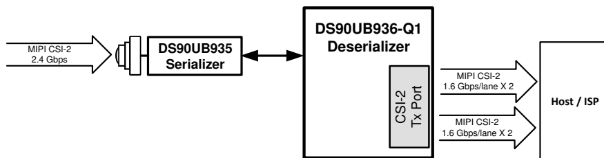
8-14. DS90UB935-Q1 Sensor Data Replicated onto 2x 2-Lane CSI-2
