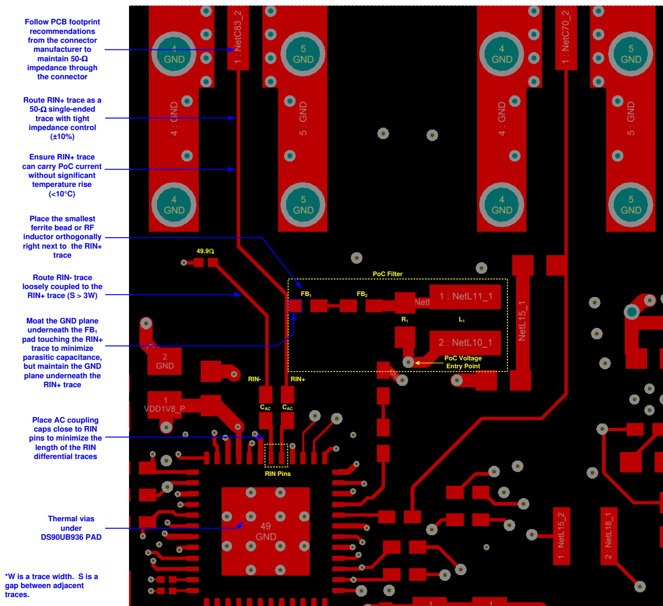
FIG 10-1. DS90UB936-Q1 PCB Layout Example: FPD-Link III Signal Traces and PoC Filter
