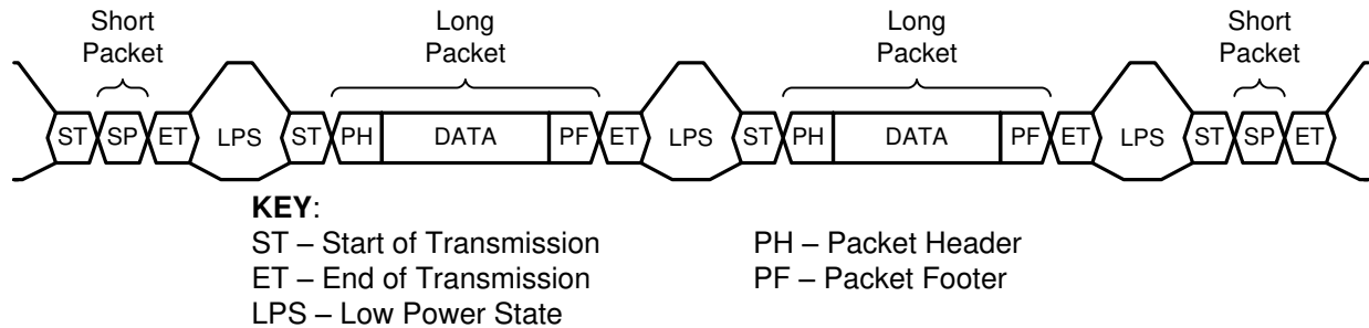
☒ 7-8. CSI-2 Protocol Layer With Short and Long Packets
