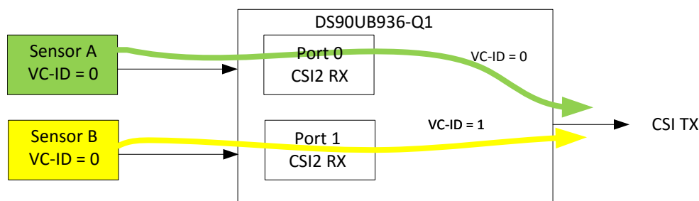
FIG 7-12. VC-ID Mapping Example 1
