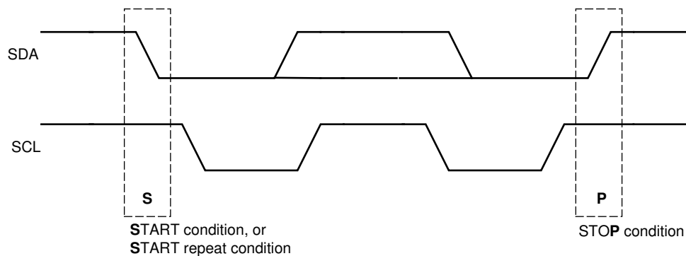
7-24. START and STOP Conditions
