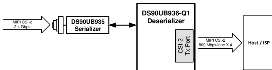
8-13. One DS90UB935-Q1 Sensor Data onto CSI-2 Over 1 Port
