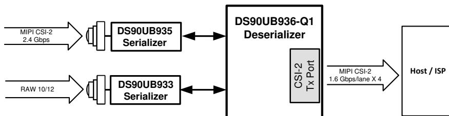
8-15. One DS90UB935-Q1 and One DS90UB933-Q1 Sensor Data Combined to One CSI-2 Output
