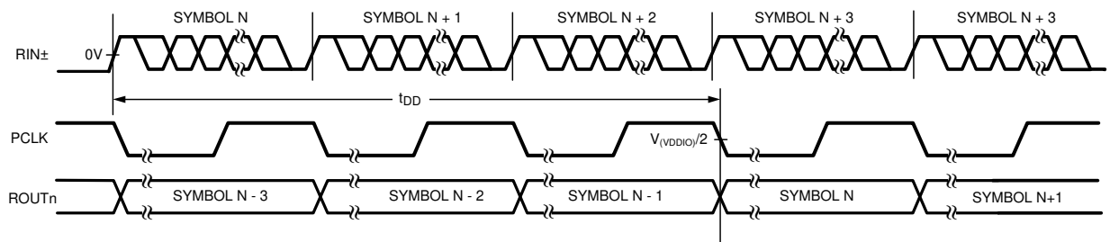
4-6. Deserializer Delay
