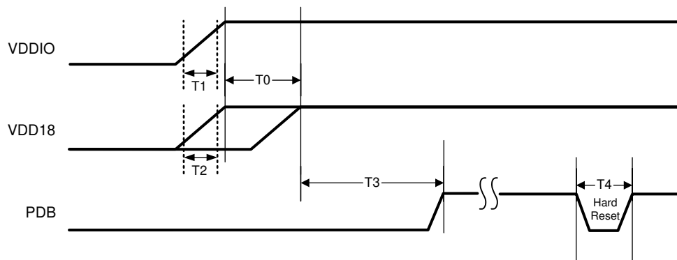
FIG 6-11. Power-Up Sequencing
