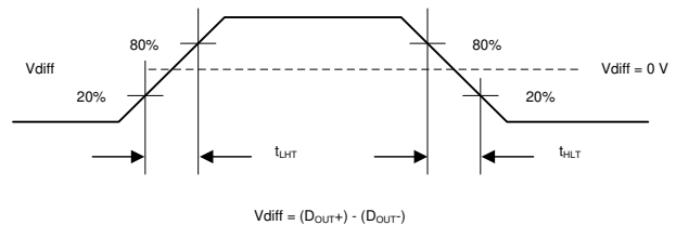
FIG 6-3. Serializer CML Output Load and Transition Times
