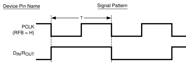
FIG 6-2. "Worst Case" Test Pattern for Power Consumption
