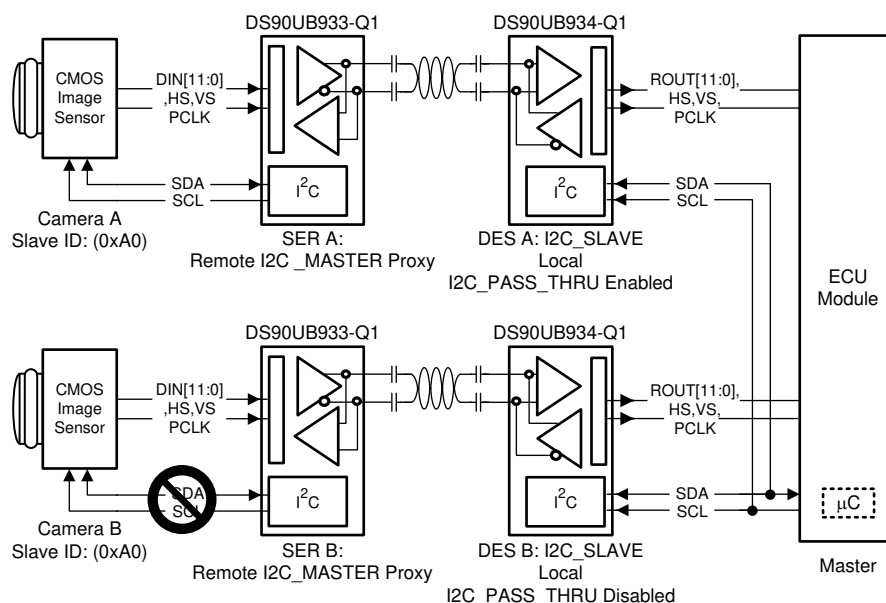
7-13. I2C Pass-Through
