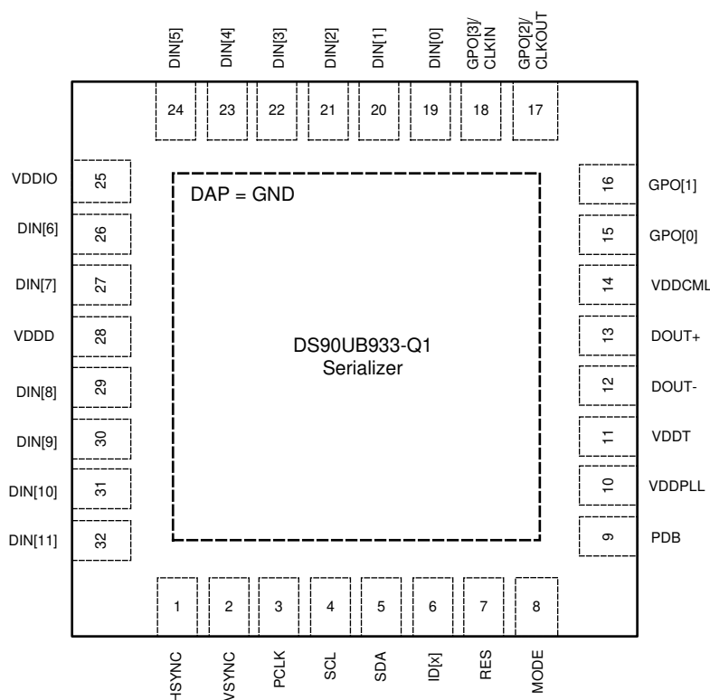
5-1. RTV Package 32-Pin WQFN Top View
