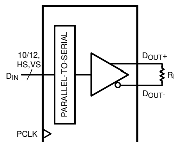
FIG 6-4. Measurement Setup Serializer CML Output Load and Transition Times
