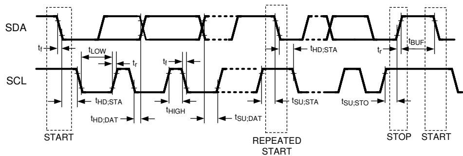
FIG 6-1. Bidirectional Control Bus Timing
