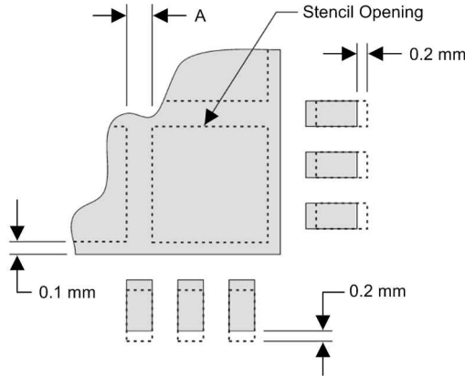
図 10-1. No Pullback WQFN, Single Row Reference Diagram
