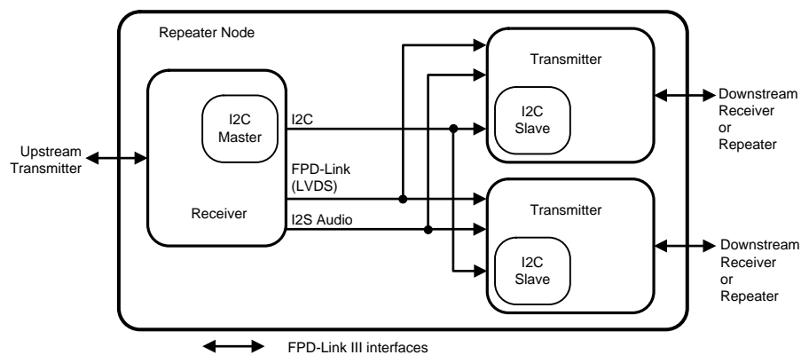
Figure 30. 1:2 Repeater Configuration
