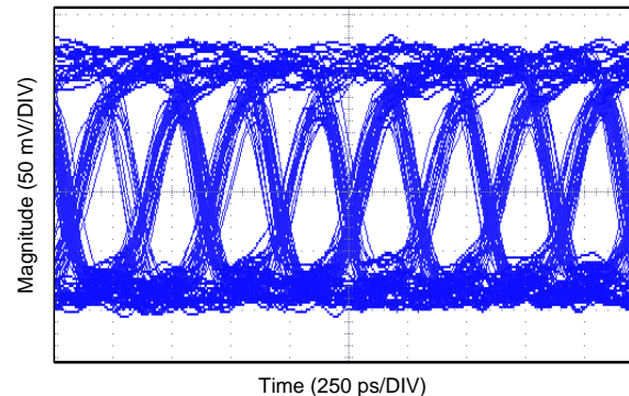
Figure 40. CMLOUT of Deserializer from 96 MHz Input Clock
