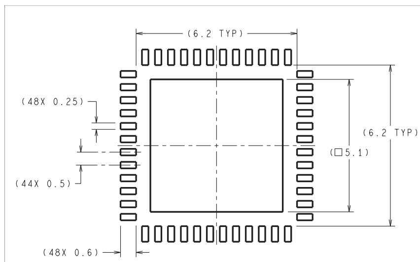
Figure 43. 48-Pin WQFN Stencil Example of Via and Opening Placement
