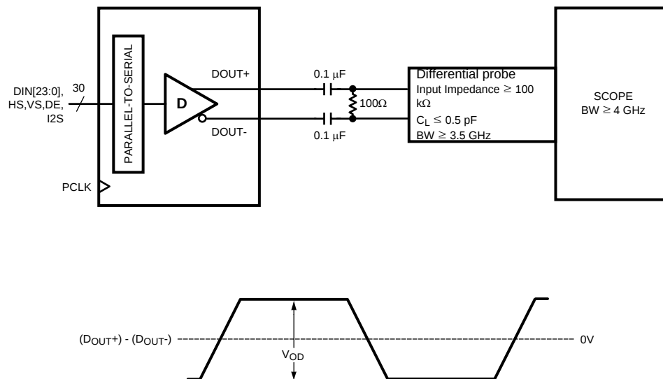
Figure 1. Serializer Differential V_{\text{OD}} DC Output
