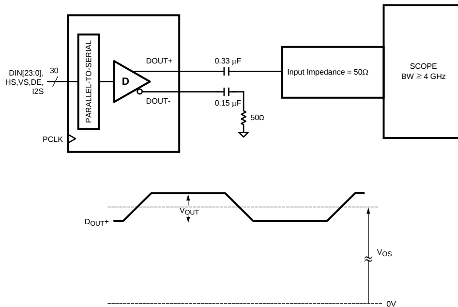
Figure 2. Serializer Single-ended V_{OUT} DC Output
