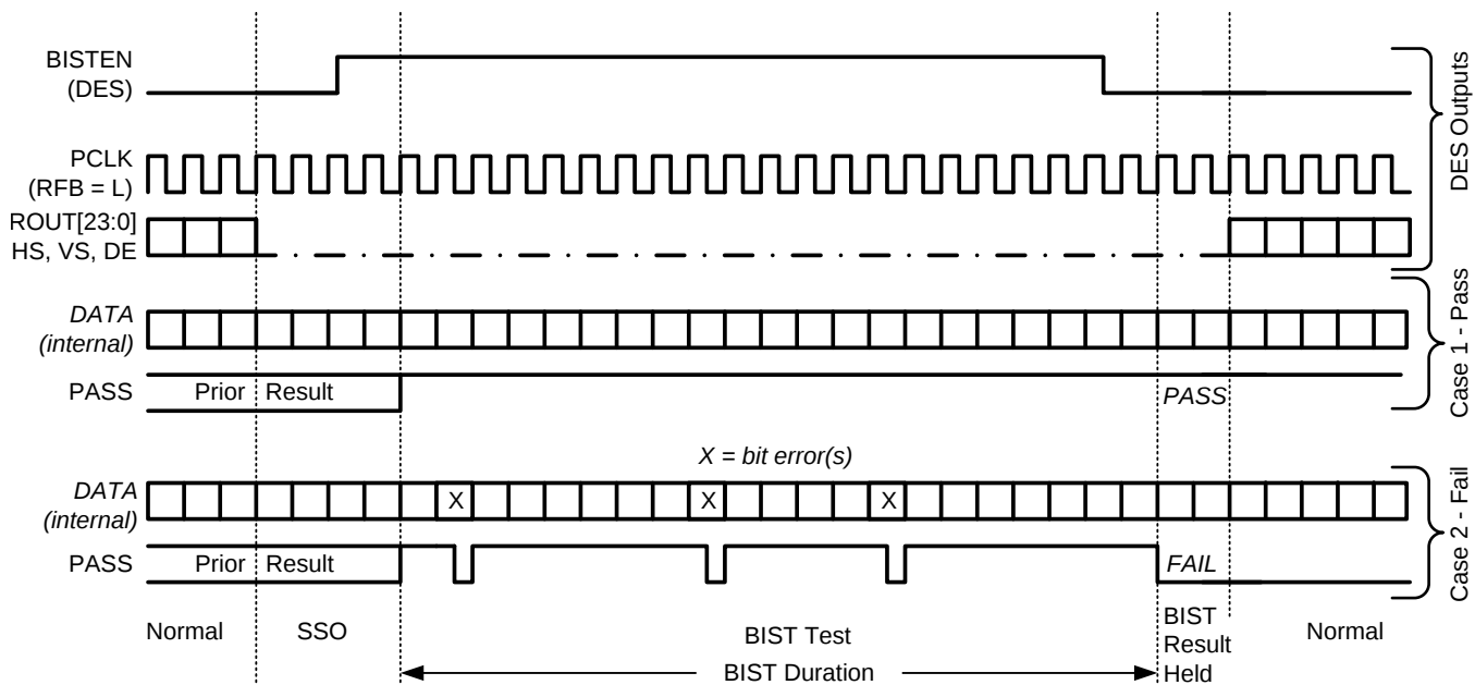
Figure 17. Bist Waveforms
