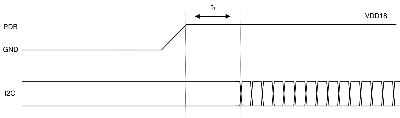
Figure 30. Suggested Timing of PDB vs. Local I2C Access for DS90UB914A-Q1
