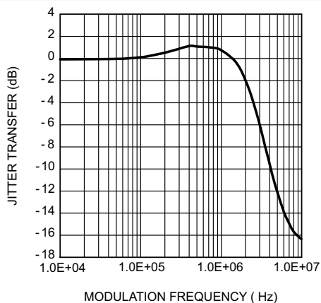
FIG 6-11. Typical Serializer Jitter Transfer Function
