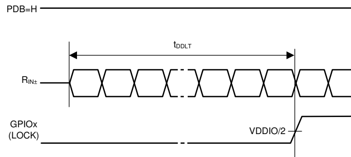
FIG 6-3. Deserializer Data Lock Time
