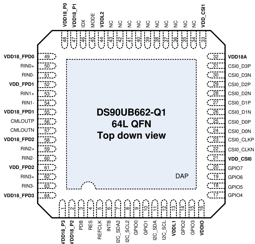
5-1. RTD Package 64-Pin VQFN (Top View)
