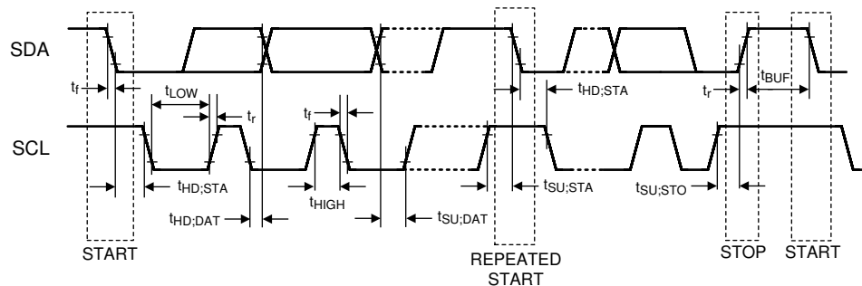
FIG 6-4. I2C Serial Control Bus Timing
