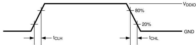
FIG 6-1. LVCMOS Transition Times
