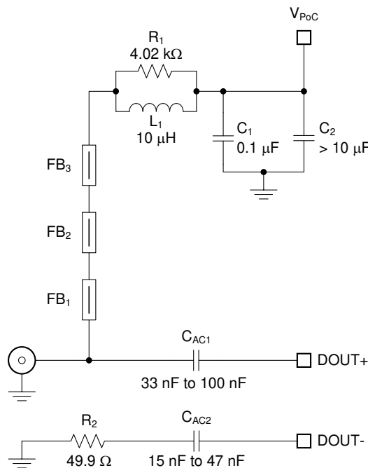
☒ 8-2. Typical PoC Network for a "4G" FPD-Link III
