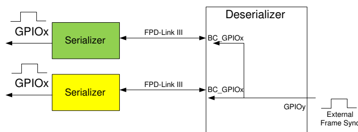
7-4. External FrameSync
