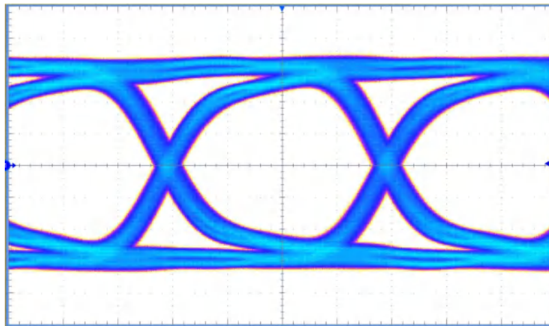
FIG 6-3. Eye Diagram at 4-Gbps FPD-Link III Forward Channel Rate From Serializer Output Vertical Scale: 100 mV/DIV Horizontal Scale: 62.5 ps/DIV
