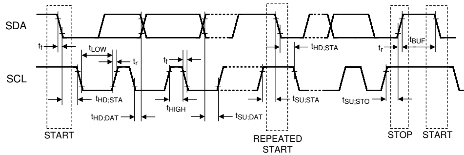
FIG 6-2. I²C Serial Control Bus Timing
