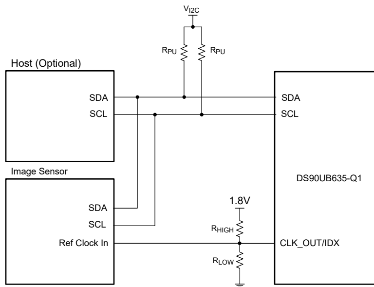
図 7-8. Circuit to Bias IDX Pin
