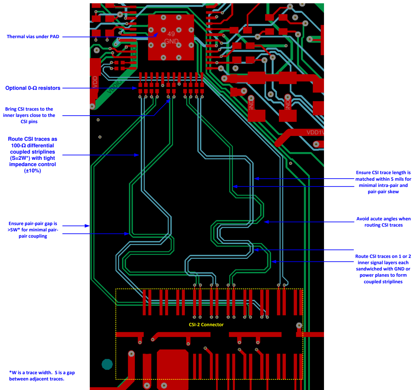
10-3. DS90UB635-Q1 Serializer CSI-2 Traces PCB Layout Example
