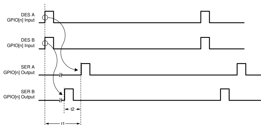
FIG 7-2. GPIO Delta Latency
