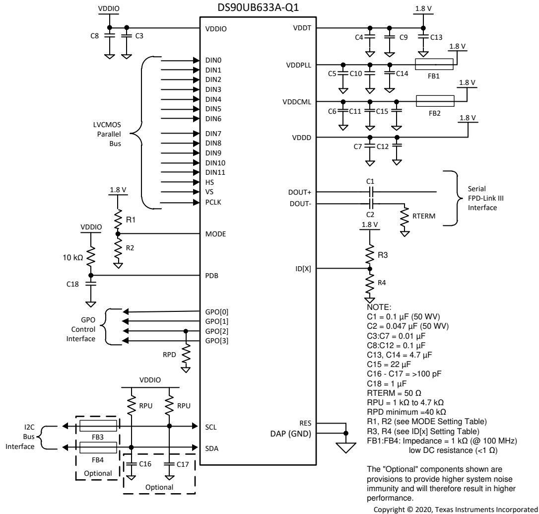
8-4. Coax Application Connection Diagram
