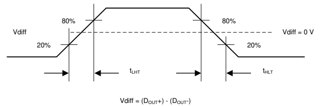
Figure 6-3. Serializer CML Output Load and Transition Times
