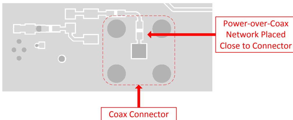
FIG 10-3. DS90UB633A-Q1 Power-over-Coax Layout
