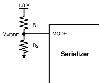
7-6. MODE Pin Configuration on DS90UB633A-Q1
