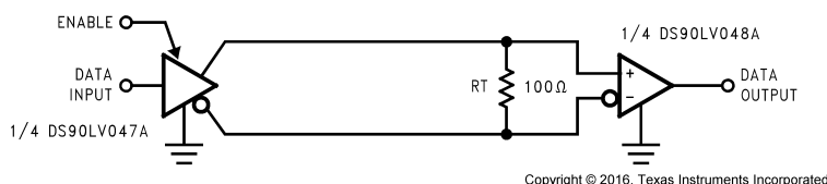
Figure 19. Balanced System Point-to-Point Application
