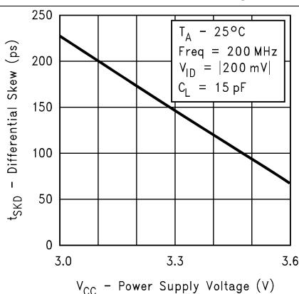
Figure 9. Differential Skew vs Power Supply Voltage
