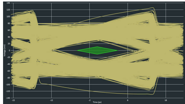
図 8-6. PCIe 5.0 Link Setup with the DS320PR410 Eye Diagram Using SigTest
