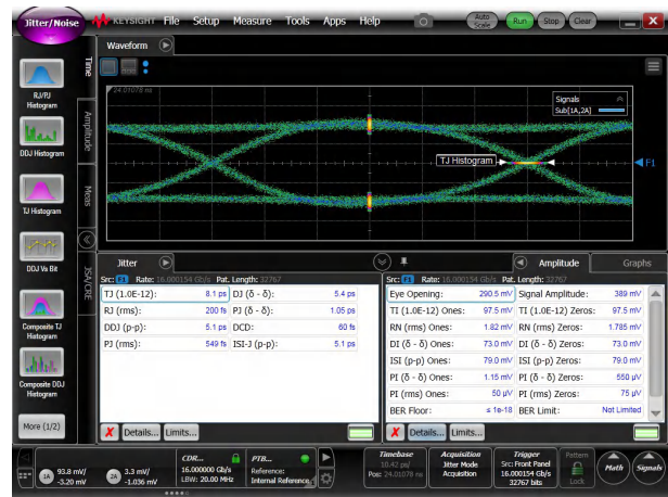
図 6-4. Through DS320PR410 and (equivalent) traces at 16 Gbps with EQ = 0 (3 dB)
