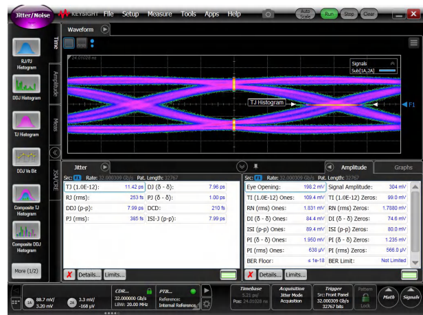
図 6-6. Through DS320PR410 and (equivalent) traces at 32 Gbps with EQ = 0 (4 dB)
