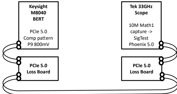
図 8-3. PCIe 5.0 Link Baseline Setup Without Redriver the Link Elements
