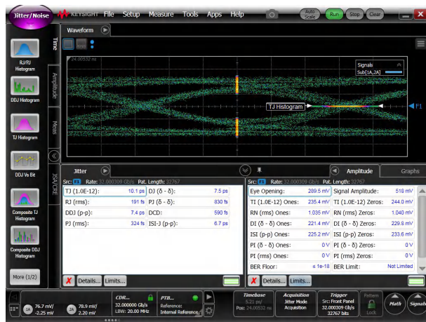
図 6-5. Through Baseline Calibration Trace (no redriver) Setup at 32 Gbps
