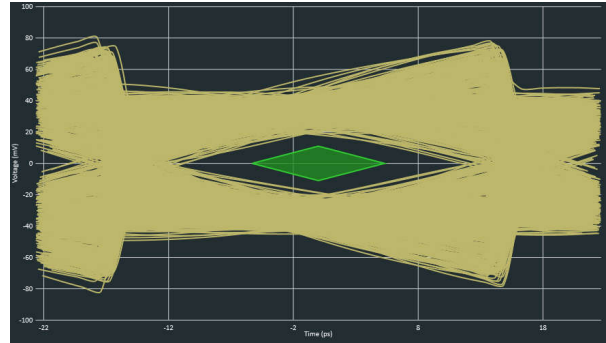
図 8-4. PCIe 5.0 link Baseline Setup Without Redriver Eye Diagram Using SigTest
