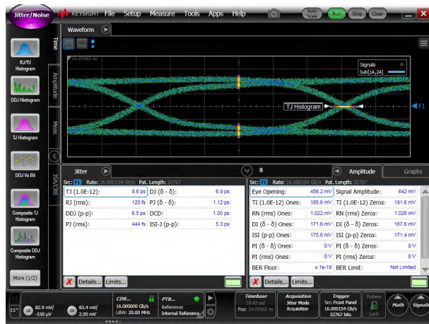
図 6-3. Through Baseline Calibration Trace (no redriver) Setup at 16 Gbps
