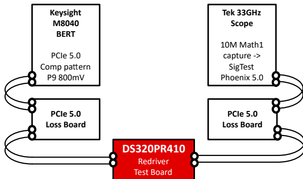
図 8-5. PCIe 5.0 Link Setup with the DS320PR410 the Link Elements
