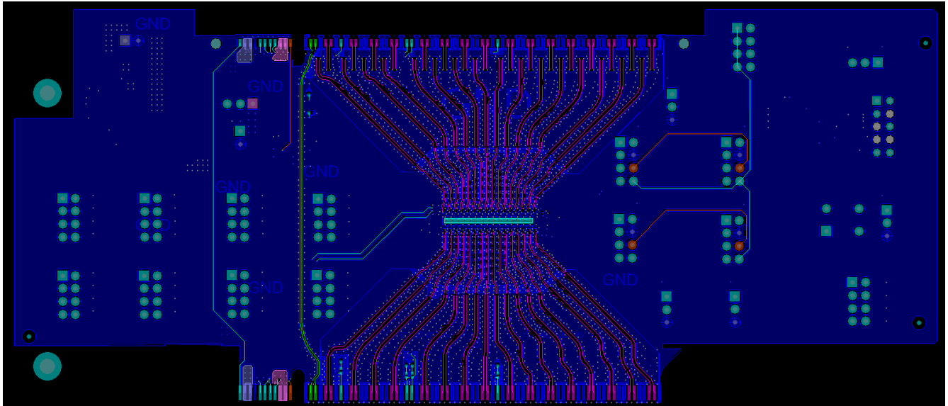
図 9-8. Bottom Layer View of TI PCIe Riser Card Using DS320PR1601 with CEM Connectors
