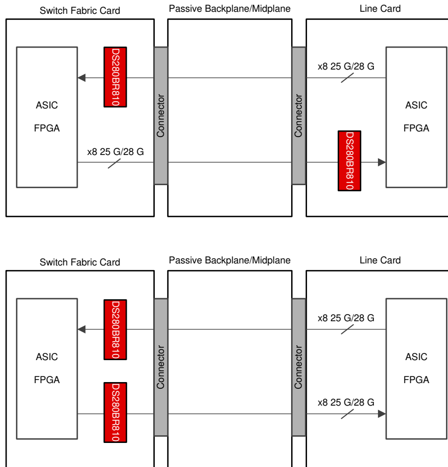
☒ 7. Typical Backplane and Mid-Plane Application Diagram
