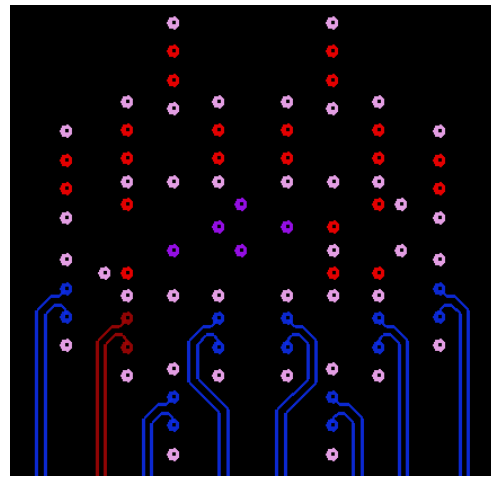
✕ 30. Internal Signal Layer 1
