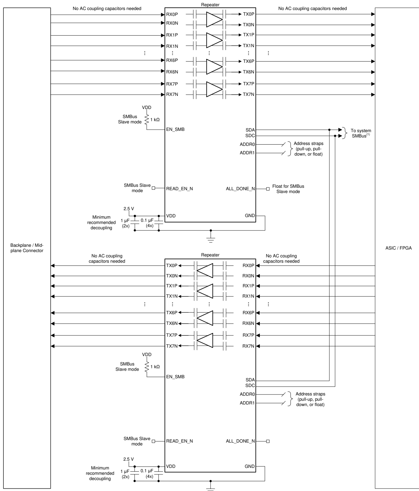
8. Typical Backplane and Mid-Plane Schematic
