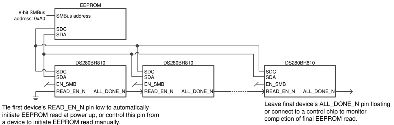
FIG 5. Example Daisy Chain for Multiple Device Single EEPROM Configuration
