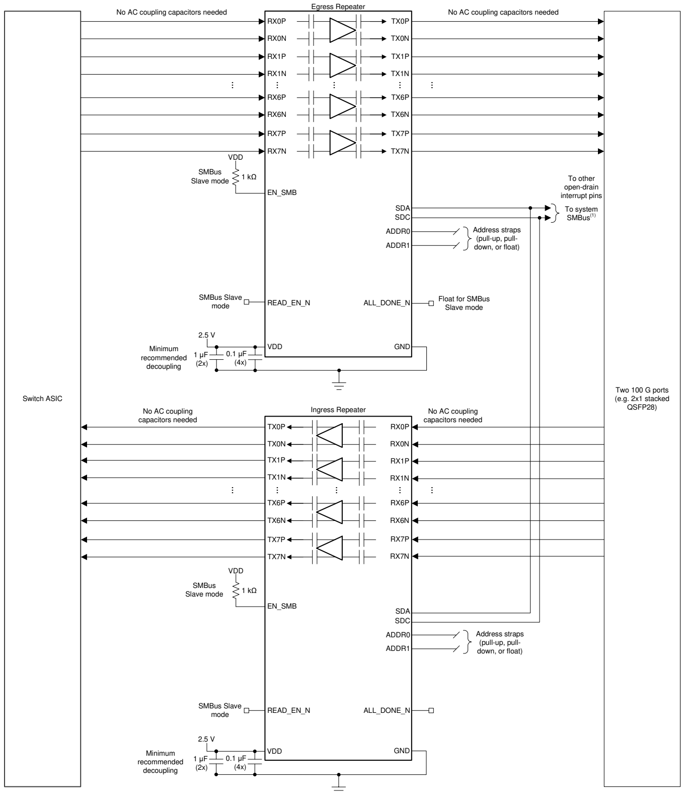
FIG 10. Typical Front-port Schematic
