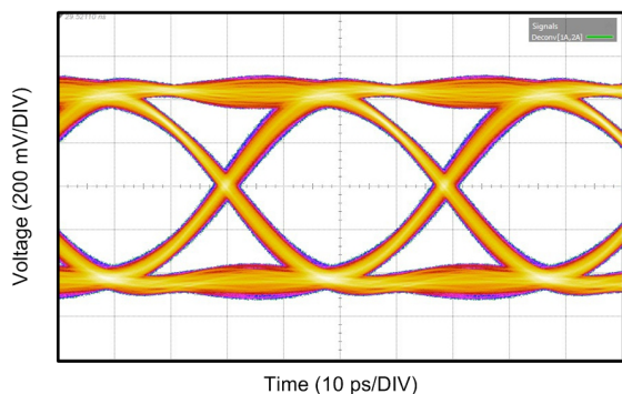
✕ 18. DS250DF810 Operating at 25.78125 Gbps
