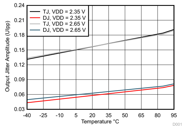
7-4. Typical Output Jitter vs Ambient Temperature at 25.78125 Gbps
