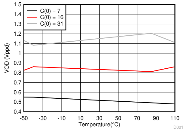
7-2. Typical VOD vs Ambient Temperature
