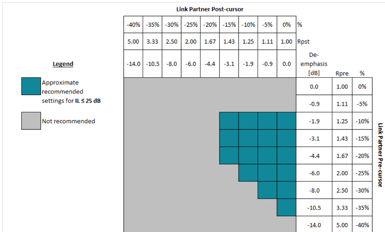
8-6. Guideline for Link Partner FIR Settings When IL ≤ 25 dB
