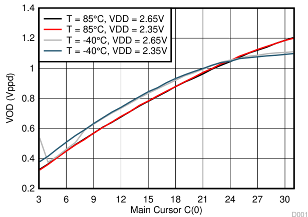
7-3. Typical VOD vs FIR Main-Cursor
