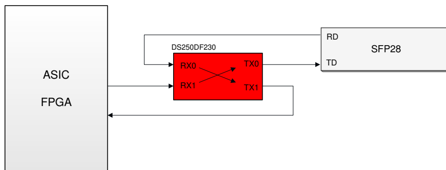
Figure 9-2. Bidirectional Application
