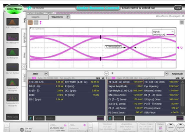
✎ 9-5. DS250DF230 Operating at 25.78125 Gbps
