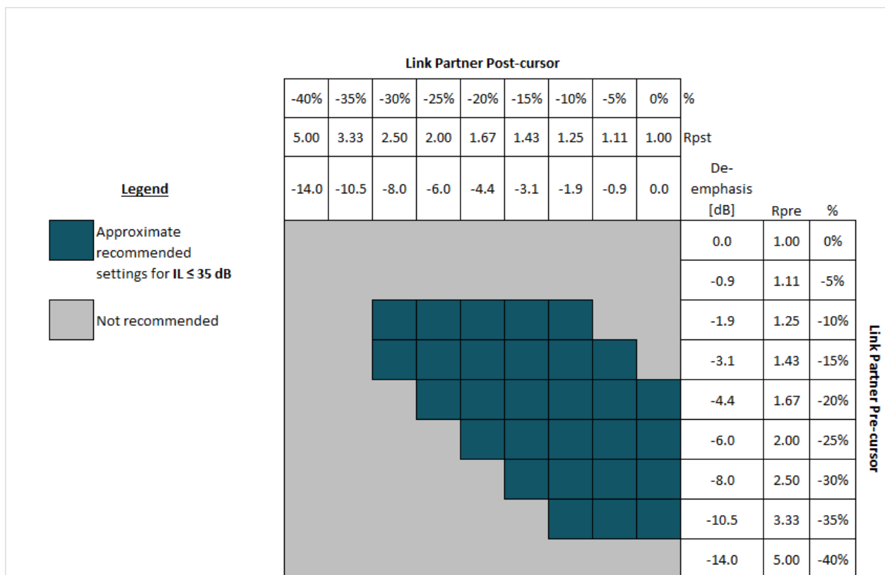
8-7. Guideline for Link Partner FIR Settings When IL ≤ 35 dB
