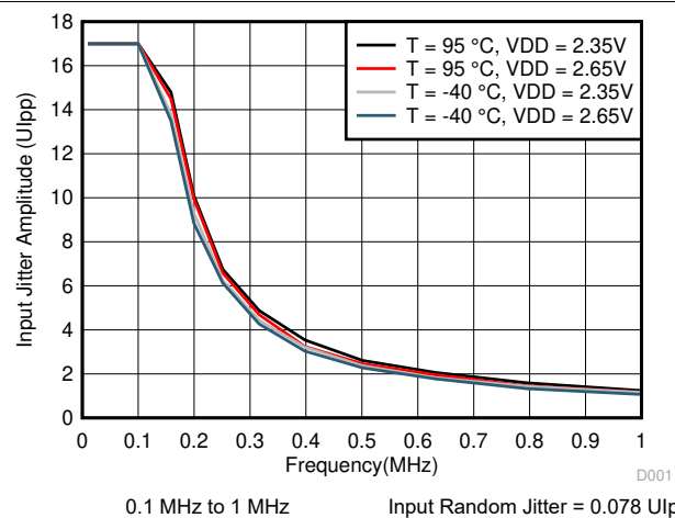
7-5. Typical Sinusoidal Input Jitter Tolerance for 30-dB Channel at 25.78125 Gbps
