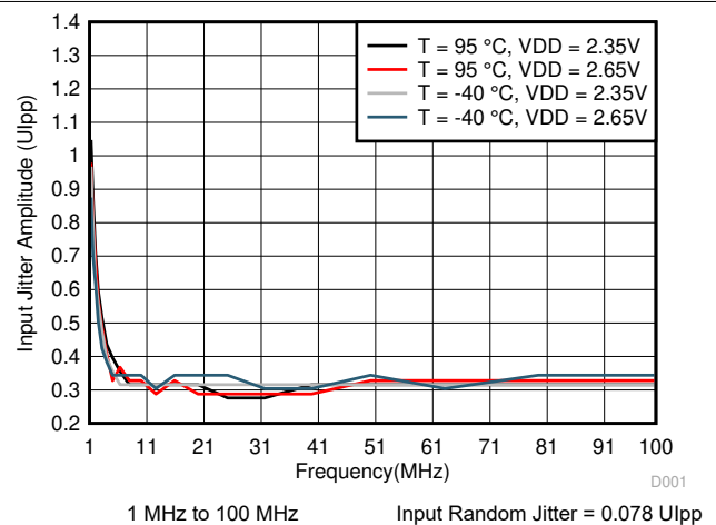
7-6. Typical Input Jitter Tolerance for 30-dB Channel at 25.78125 Gbps
