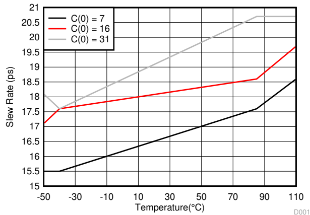
7-1. Output Transition-time vs Ambient Temperature
