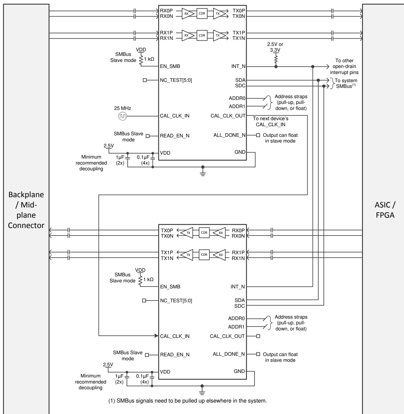
图 21. Backplane/Mid-Plane Application Schematic
