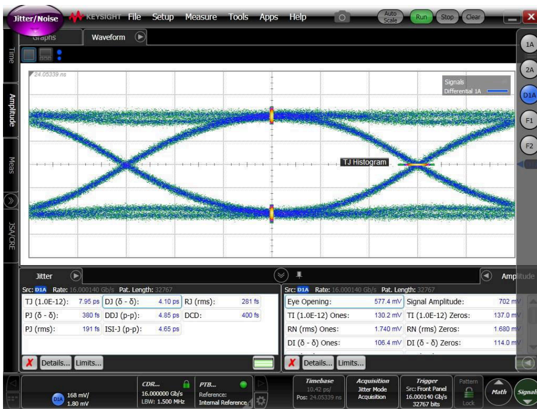
6-5. Typical Jitter Characteristics - Top: 16Gbps PRBS15 Input to the Device, Bottom: Output of the Device.
