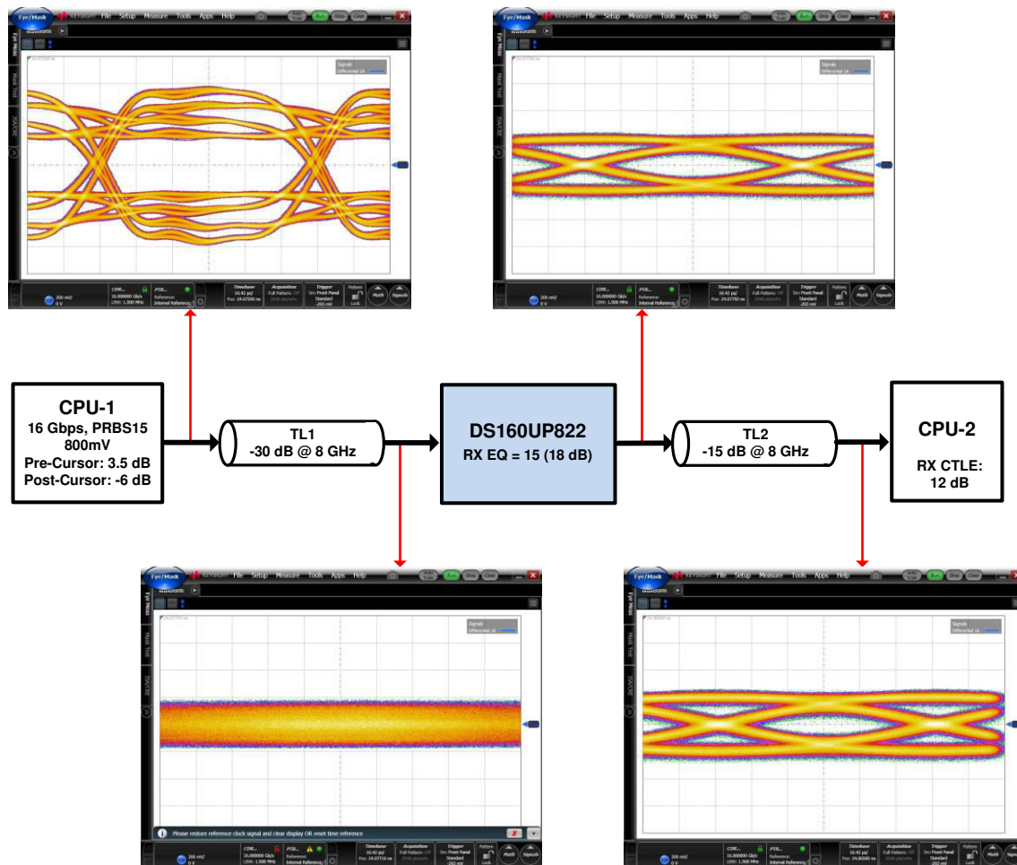
✎ 8-3. UPI 2.0 Link Reach Extension Using DS160UP822
