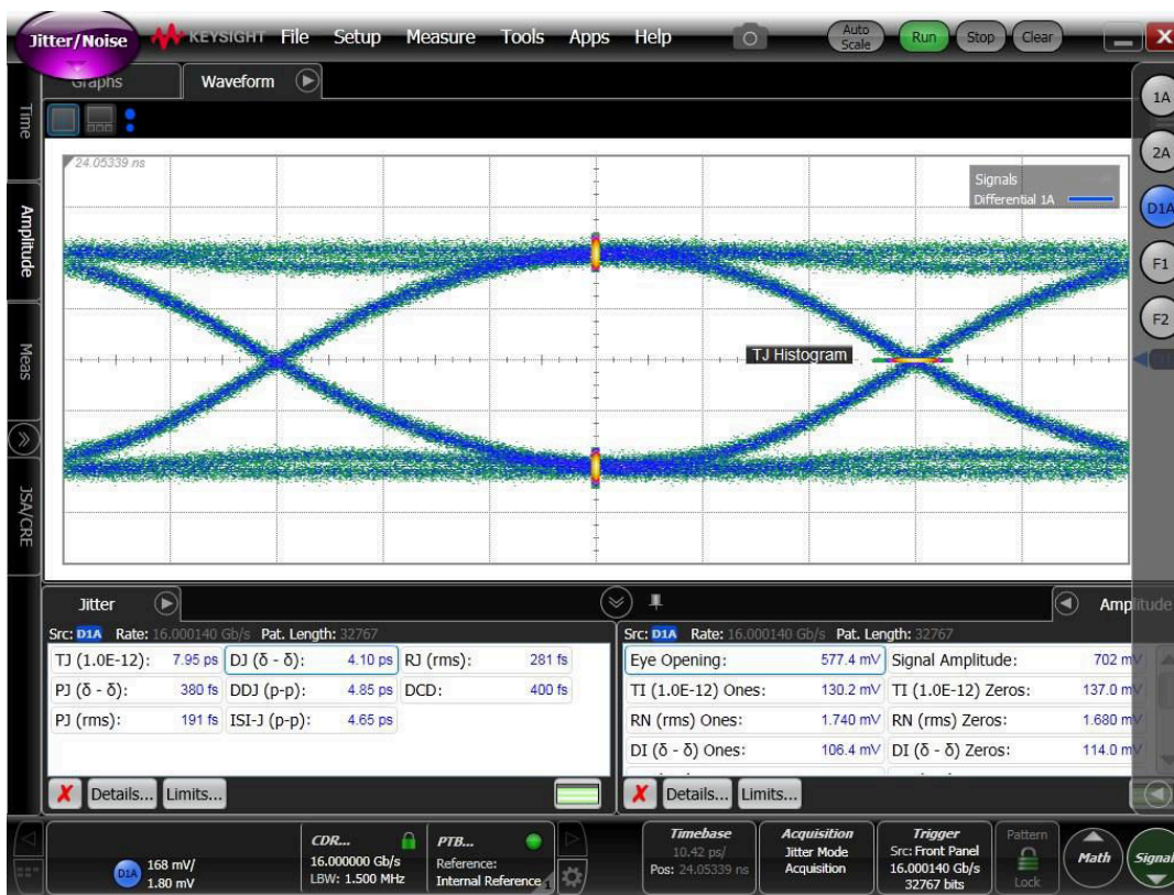
6-5. Typical Jitter Characteristics - Top: 16Gb/s PRBS15 Input to the Device, Bottom: Output of the Device.
