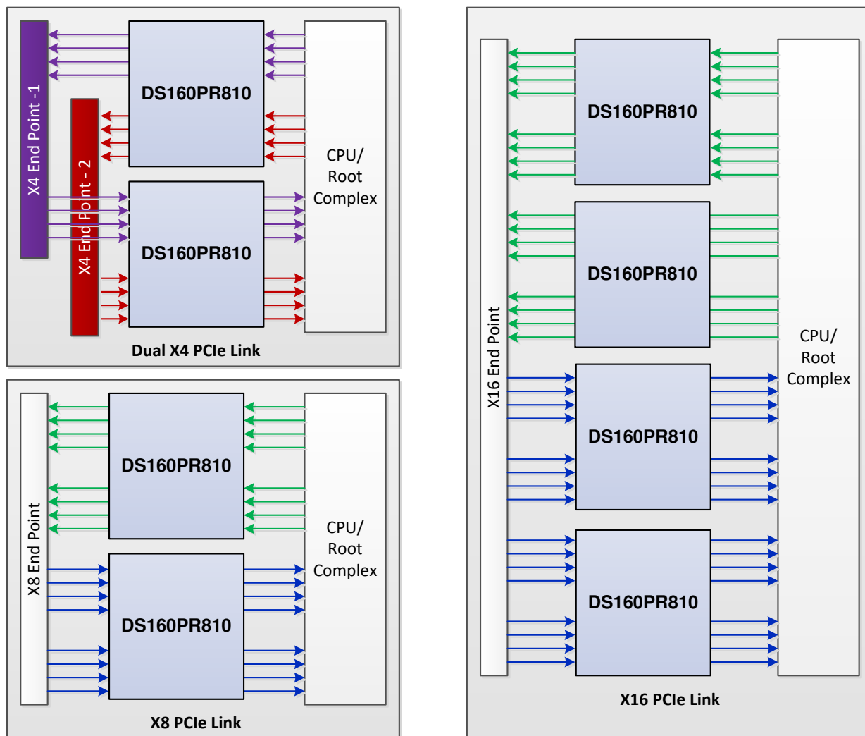
FIG 8-1. PCI Express x4, x8 and x16 use cases using DS160PR810
