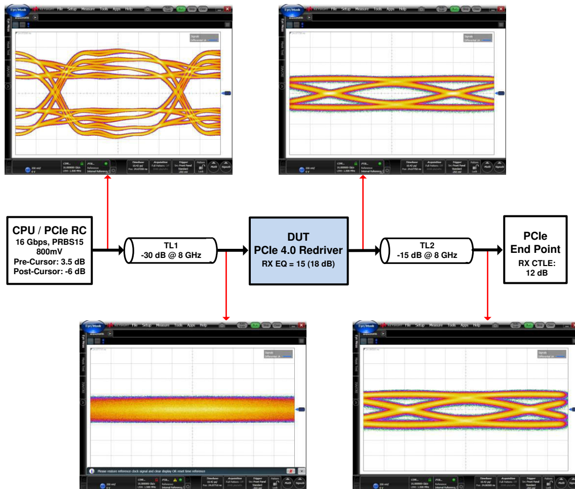
✎ 8-5. PCIe 4.0 Link Reach Extension Using DS160PR810
