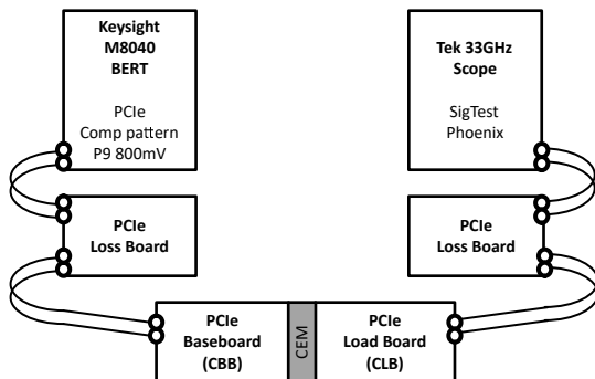
8-3. PCIe 4.0 Link Baseline Setup Without Redriver – Link Elements
