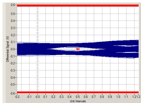
8-4. PCIe 4.0 link Baseline Setup Without Redriver – Eye Diagram Using SigTest
