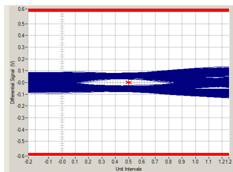
8-6. PCIe 4.0 Link Setup with the DS160PR1601 – Eye Diagram Using SigTest
