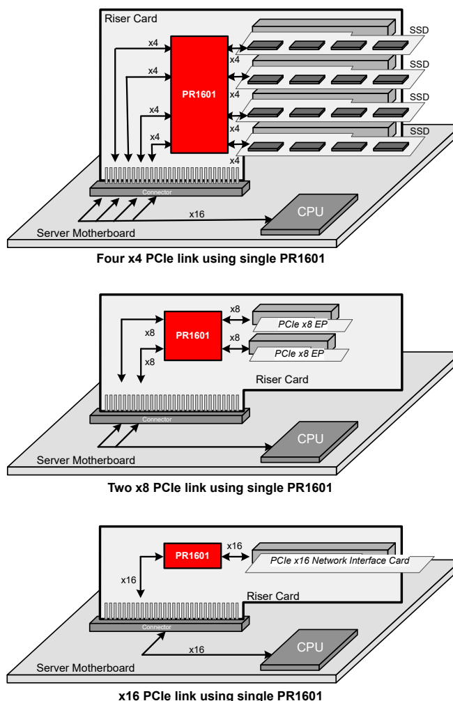
8-1. PCI Express x4, x8, and x16 Implementation Using DS160PR1601
