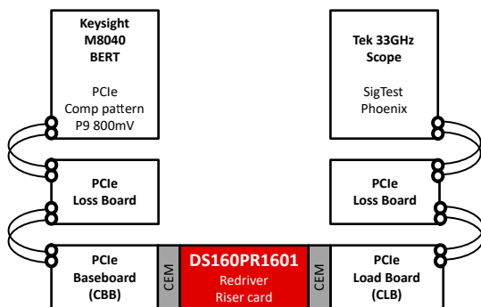
8-5. PCIe 4.0 Link Setup with the DS160PR1601 – the Link Elements
