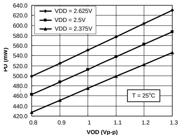
Figure 8. Power Dissipation (PD) vs. Output Differential Voltage (VOD)
