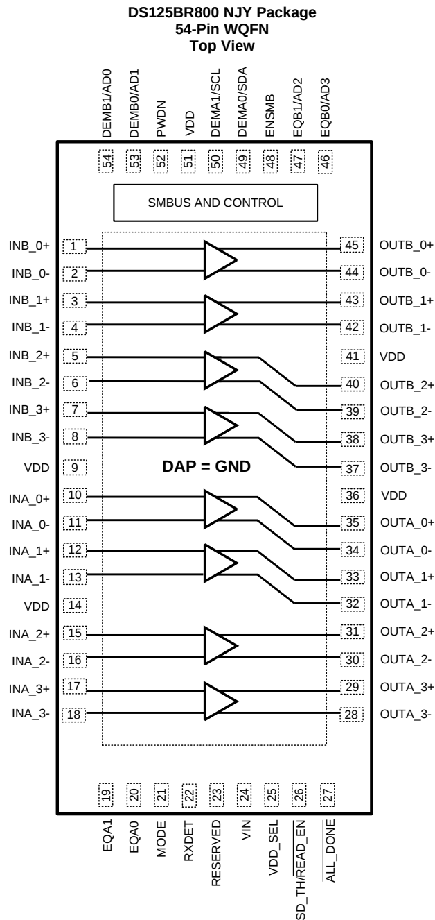
Pin Functions (1)
