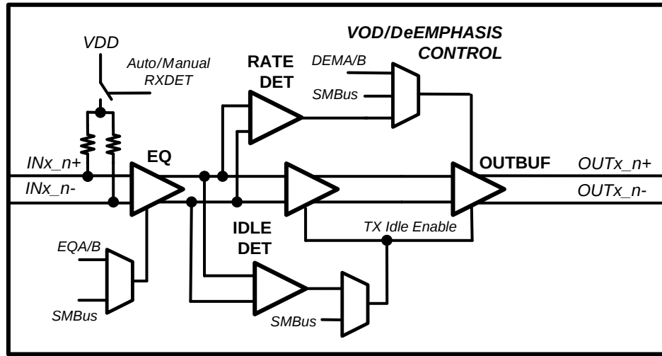
Figure 8. Block Diagram - Detail View of Channel (1 of 8)
