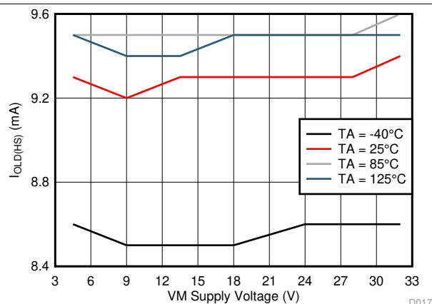
Figure 18. High-Side Open-Load Detection Current ( I_{OL(D)} ) vs Supply Voltage ( V_{VM} )
