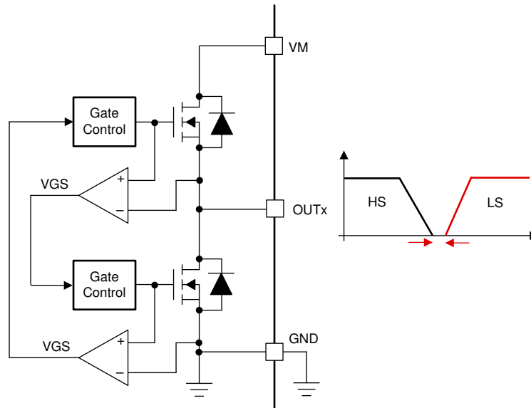
42. Cross Conduction Protection
