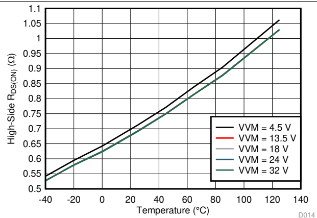
Figure 15. High Side On-State Resistance ( R_{DS(ON)} ) vs Ambient Temperature ( T_A )
