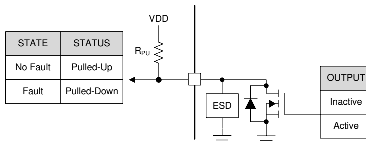
Figure 47. Open Drain Output Pin Structure (nFAULT)
