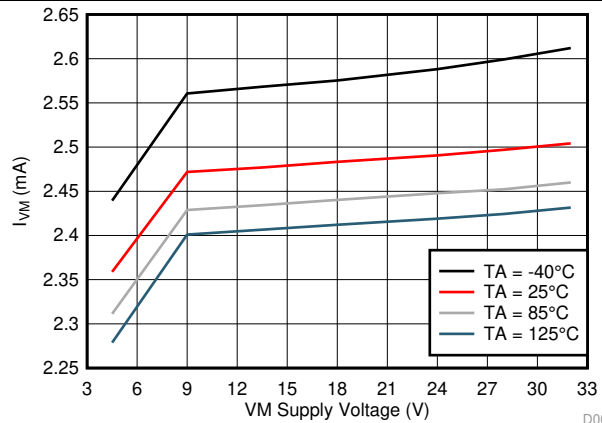
FIG 10. VM Operating Mode Current ( I_{VM} ) vs Supply Voltage ( V_{VM} )
