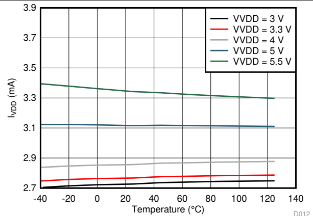
FIG 13. VDD Operating Mode Current ( I_{VDD\_O} ) vs Ambient Temperature ( T_A )
