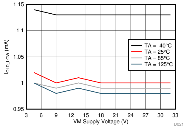
FIG 22. Low open-load detection current ( I_{OLDS\_LOW} ) vs supply voltage ( V_{VM} )
