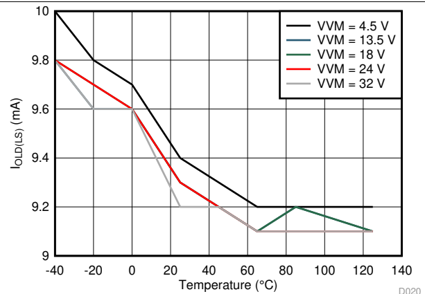
FIG 21. Low-Side Open-load Detection Current ( I_{OLDS} ) vs Ambient Temperature ( T_A )
