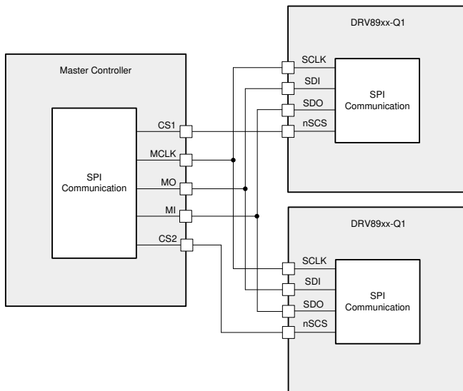
図 62. SPI Operation Without Daisy Chain
