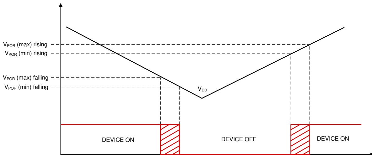
☒ 51. VDD UVLO Operation
