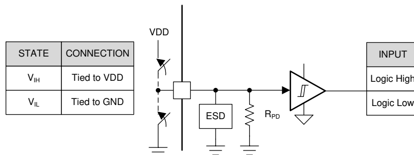
Figure 45. Logic Level Input Pin Structure (nSLEEP, SCLK and SDI)
