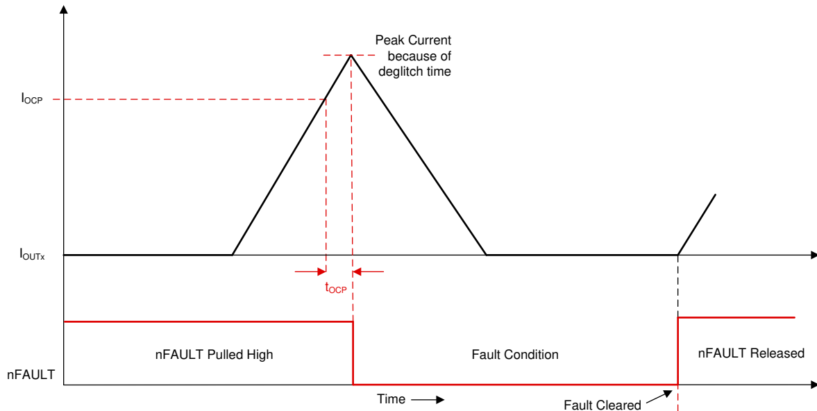
図 52. Over Current Protection
