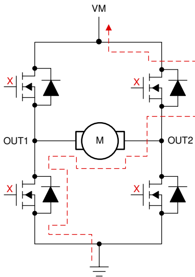
Figure 26. Continuous Mode (Coast - From Forward Direction)
