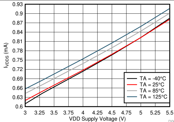
FIG 8. VDD Standby Mode Current ( I_{VDD\_S} ) vs Supply Voltage ( V_{VDD} )
