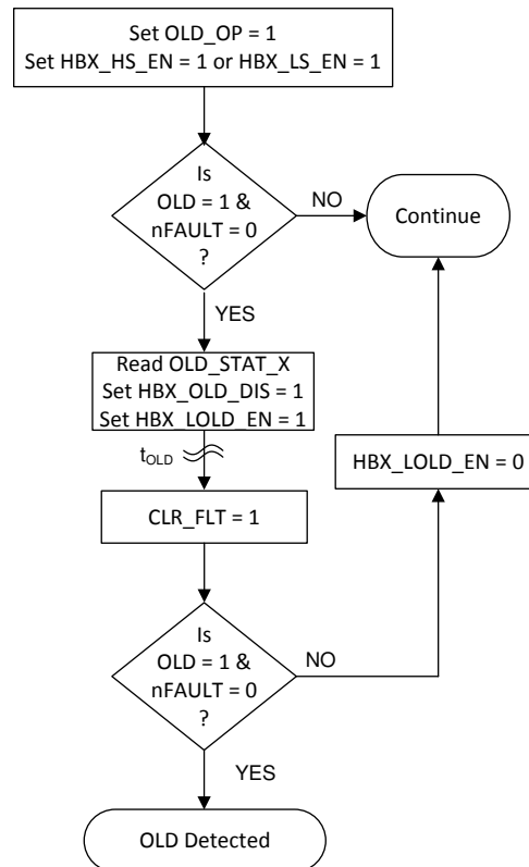
✎ 59. Flowchart for Enabling Low-Current OLD (Continuous Mode)
