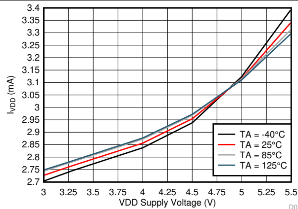
FIG 12. VDD Operating Mode Current ( I_{VDD\_O} ) vs Supply Voltage ( V_{VDD} )
