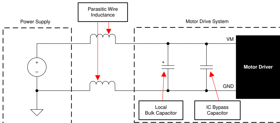
FIG 154. Motor Drive Power Supply Parasitic Example
