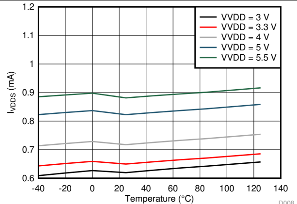
FIG 9. VDD Standby Mode Current ( I_{VDD\_S} ) vs Ambient Temperature ( T_A )
