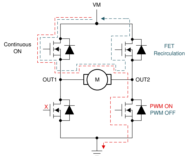
31. PWM Mode (Synchronous Rectification = ON)
