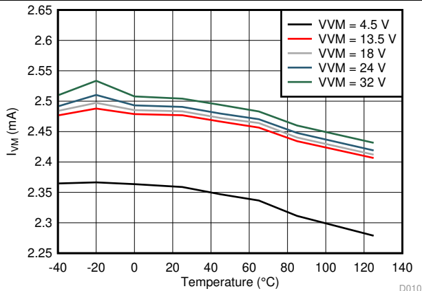
FIG 11. VM Operating Mode Current ( I_{VM} ) vs Ambient Temperature ( T_A )
