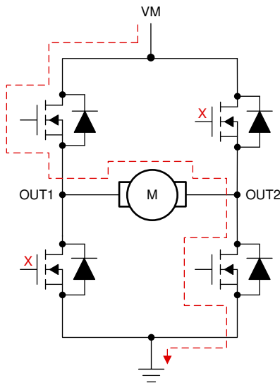
Figure 24. Continuous Mode (Forward Direction)
