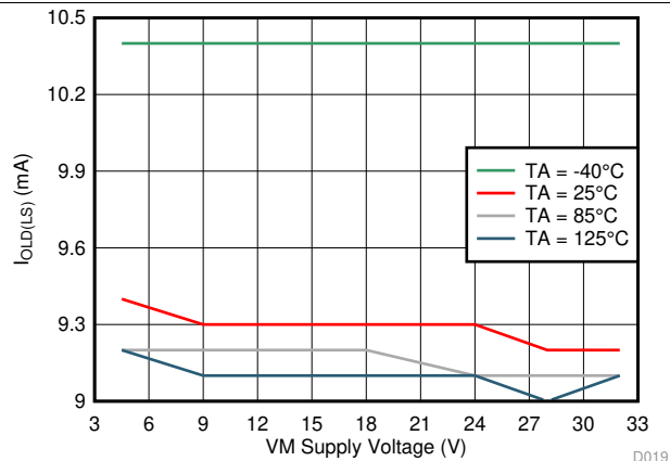
FIG 20. Low-Side Open-Load Detection Current ( I_{OLDS} ) vs Supply Voltage ( V_{VM} )
