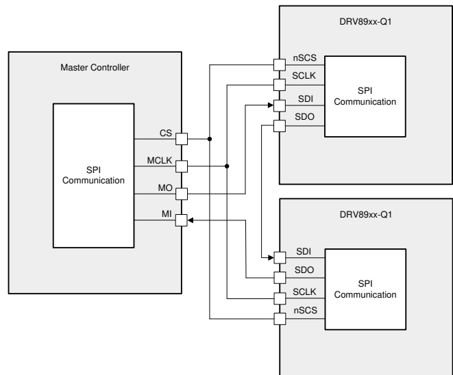
図 63. SPI Operation With Daisy Chain
