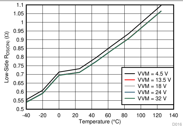
Figure 17. Low-Side On-State Resistance ( R_{DS(ON)} ) vs Ambient Temperature ( T_A )
