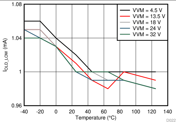
FIG 23. Low open-load detection current ( I_{OLD\_LOW} ) vs ambient temperature ( T_A )
