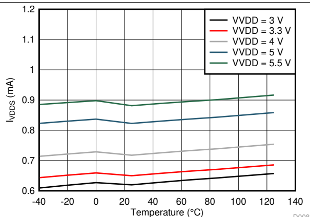
FIG 9. VDD Standby Mode Current ( I_{VDD\_S} ) vs Ambient Temperature ( T_A )
