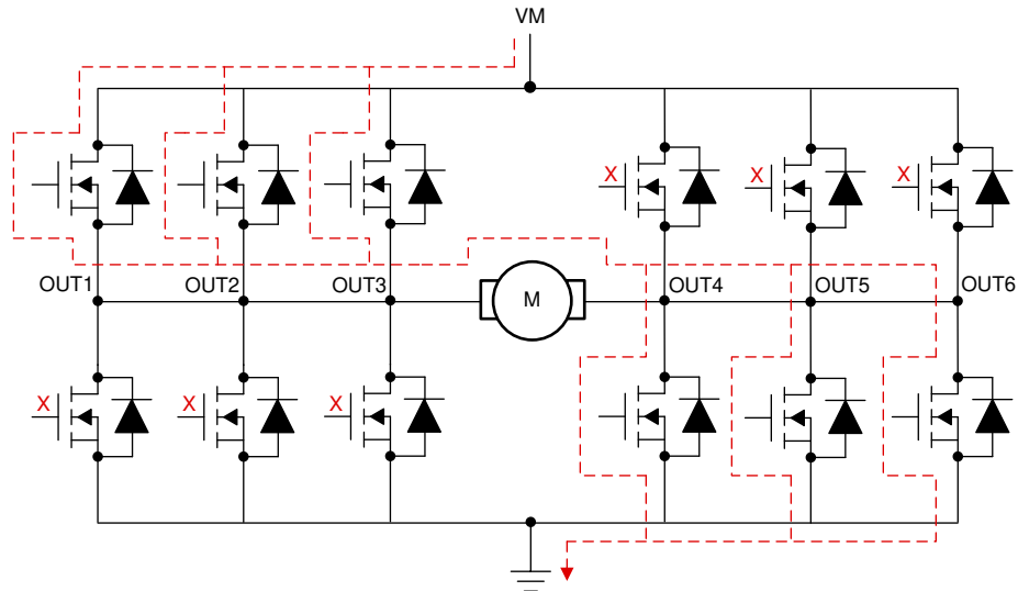
Figure 32. Parallel Mode (Forward Direction)
