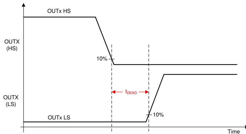
Figure 43. Dead Time
