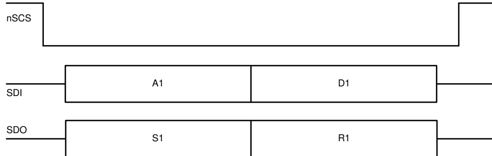
Figure 61. SPI Data Frame
