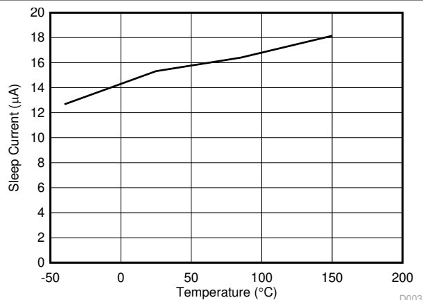
FIG 6-4. Sleep Current (I VM(Q) ) vs Temperature
