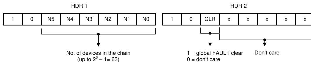
7-20. Header Bytes
