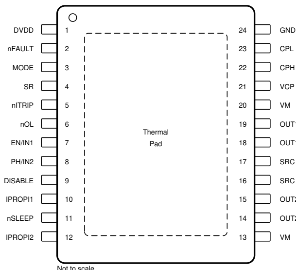
FIG 5-1. DRV8873H-Q1 PWP PowerPAD Package 24-Pin HTSSOP Top View
