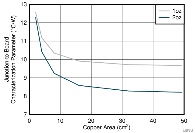
8-6. 2-Layer PCB (No Vias) Junction-to-Board Characterization Parameter vs Copper Area
