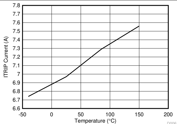
FIG 6-5. ITRIP Current vs Temperature
