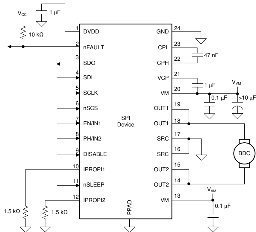
8-1. Typical Application Schematic
