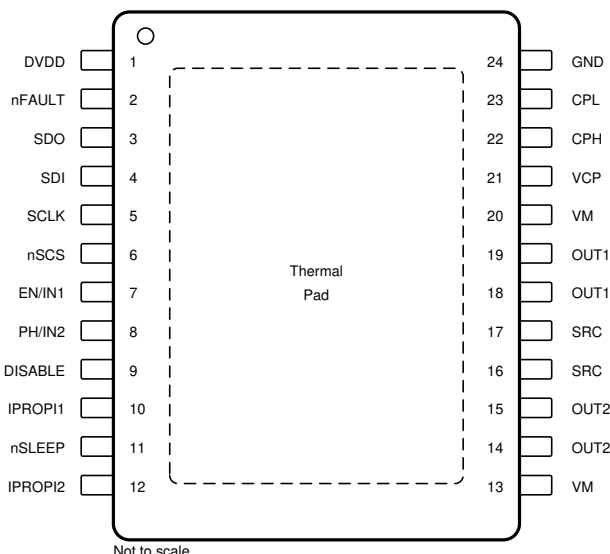
FIG 5-2. DRV8873S-Q1 PWP PowerPAD Package 24-Pin HTSSOP Top View
