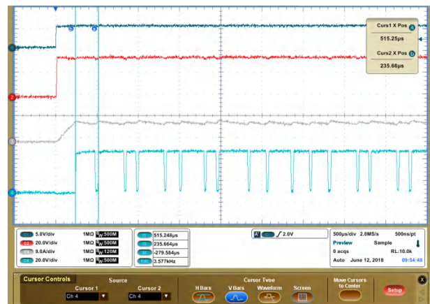
8-10. Motor Motion at Different Speeds
