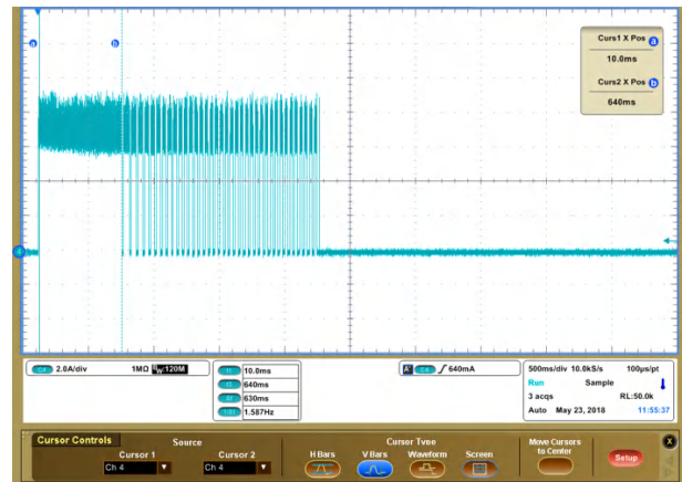
8-8. Current Regulation (ITRIP)
