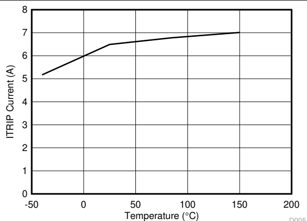
FIG 6-6. ITRIP Current vs Temperature
