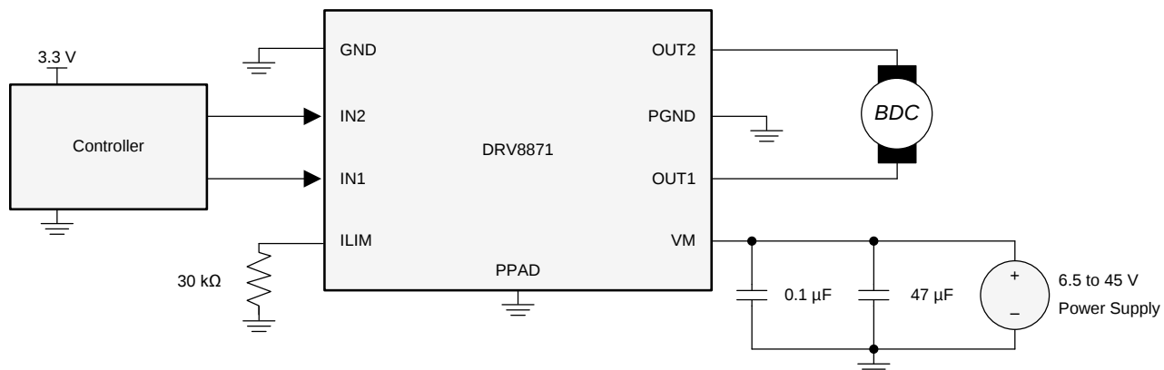
Figure 7. Typical Connections
