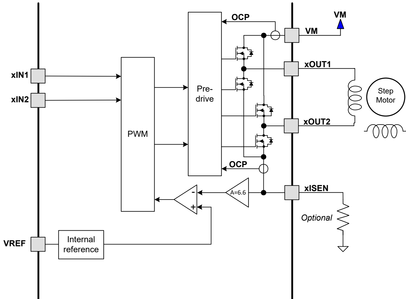
図 6-1. PWM Motor Driver Circuitry
