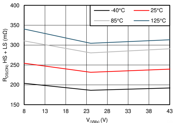
6-3. R_{DS(ON)} vs V_{VMx}
