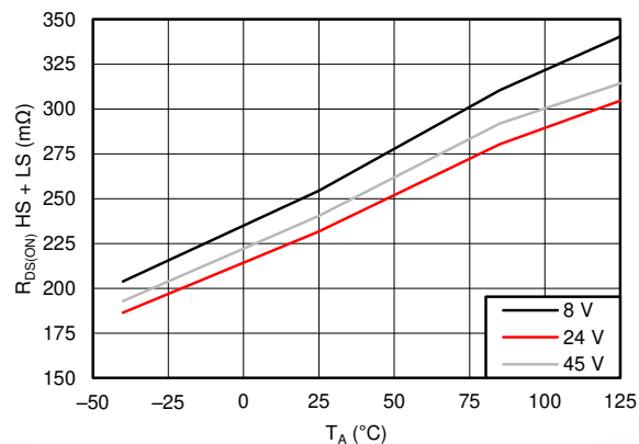
6-4. R_{DS(ON)} vs Temperature
