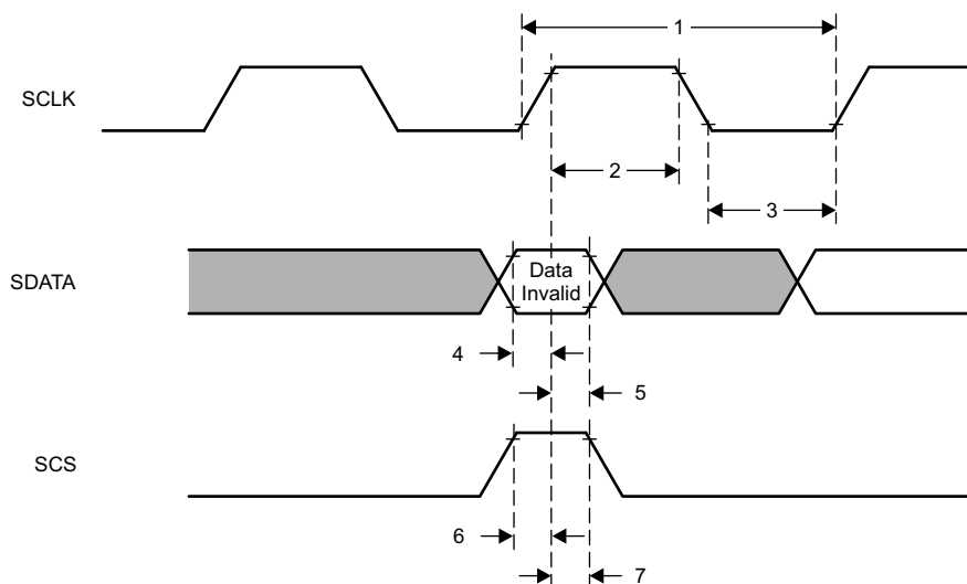
Figure 2. Timing Diagram
