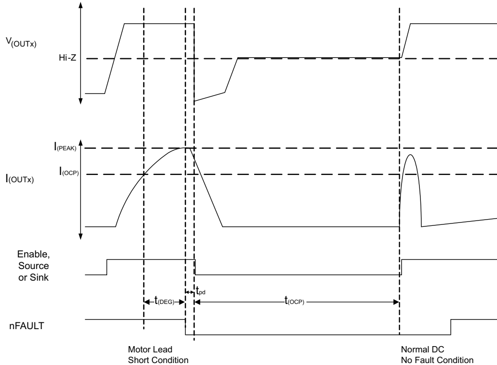
Figure 7-2. Overcurrent Control Timing
