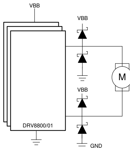
FIG 9-10. Schottky Diodes Connection
