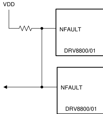
FIG 9-9. nFAULT as Wired OR
