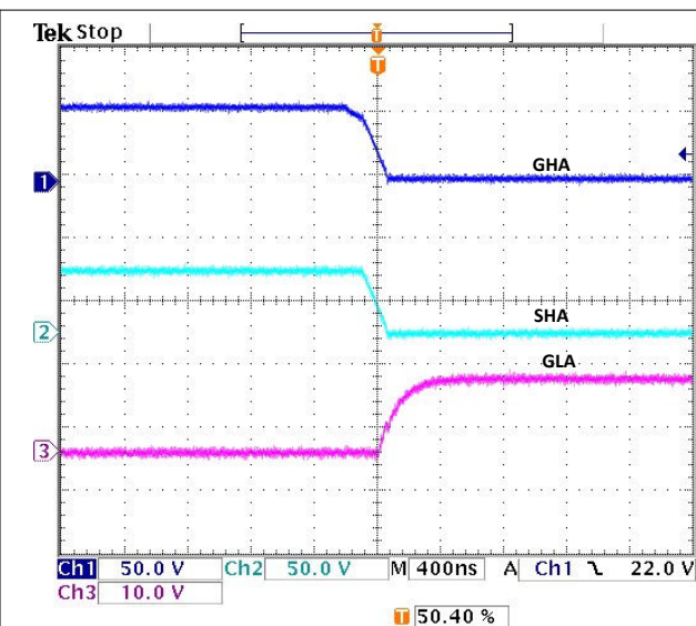
8-3. Gate voltages, SHx falling with 15 ohm gate resistor and CSD19532Q5B MOSFET
