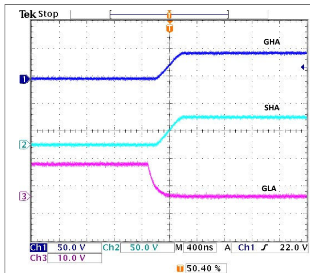
8-2. Gate voltages, SHx rising with 15 ohm gate resistor and CSD19532Q5B MOSFET
