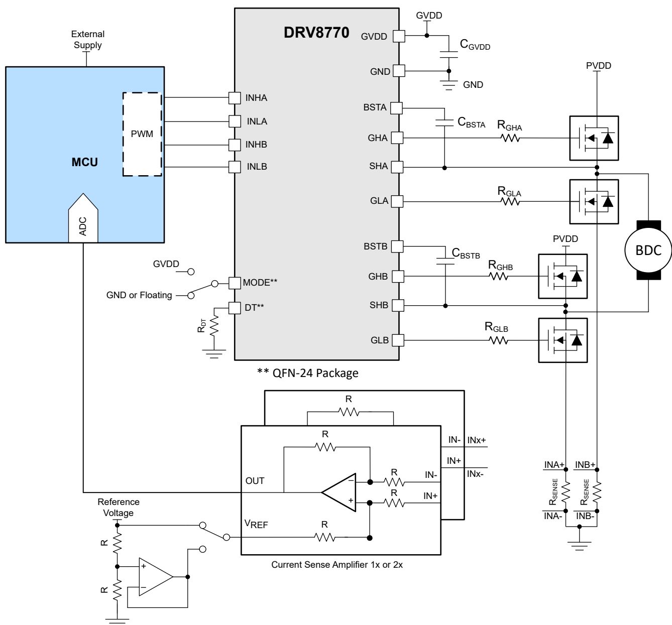
8-1. Application Schematic
